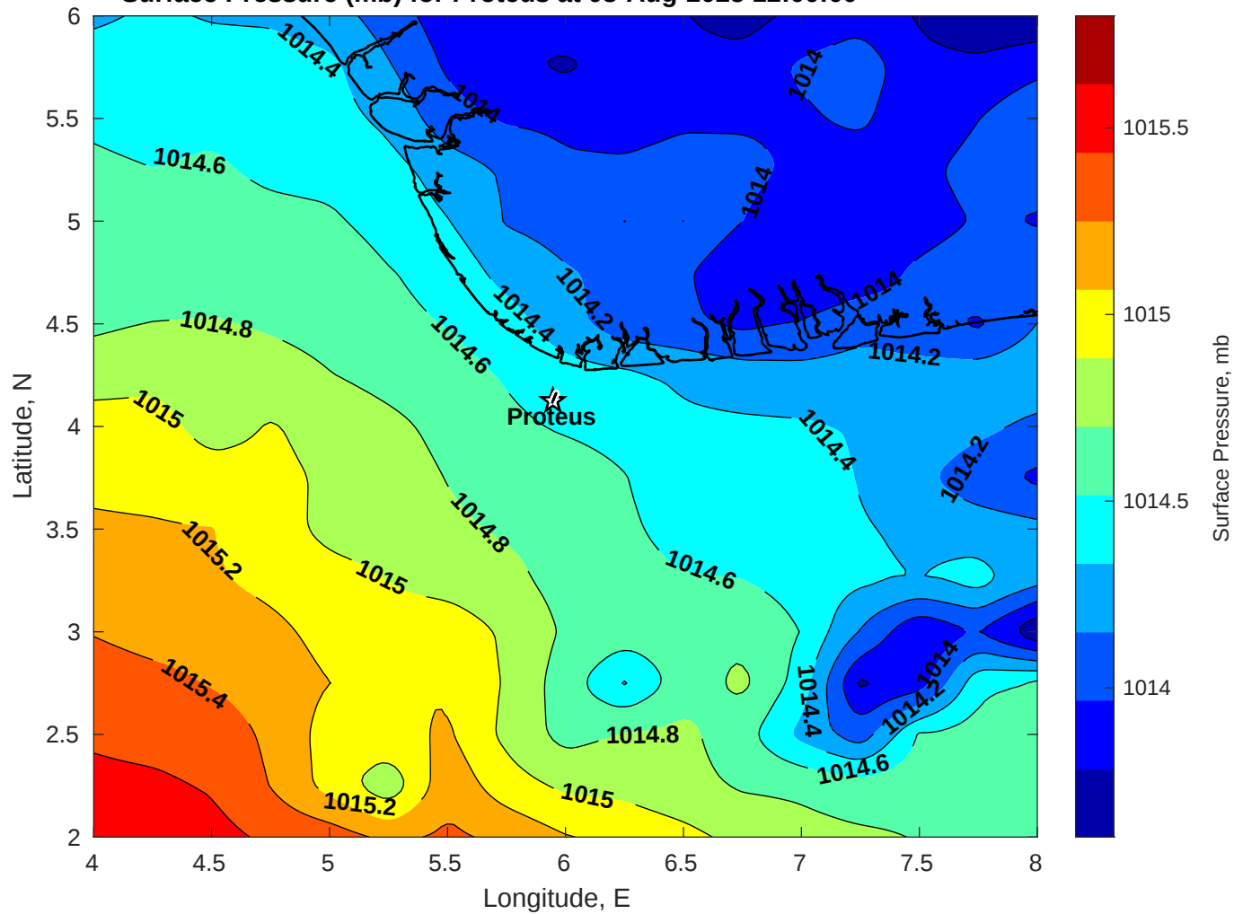
Surface Pressure (mb) for Proteus at 03-Aug-2025 12:00:00
