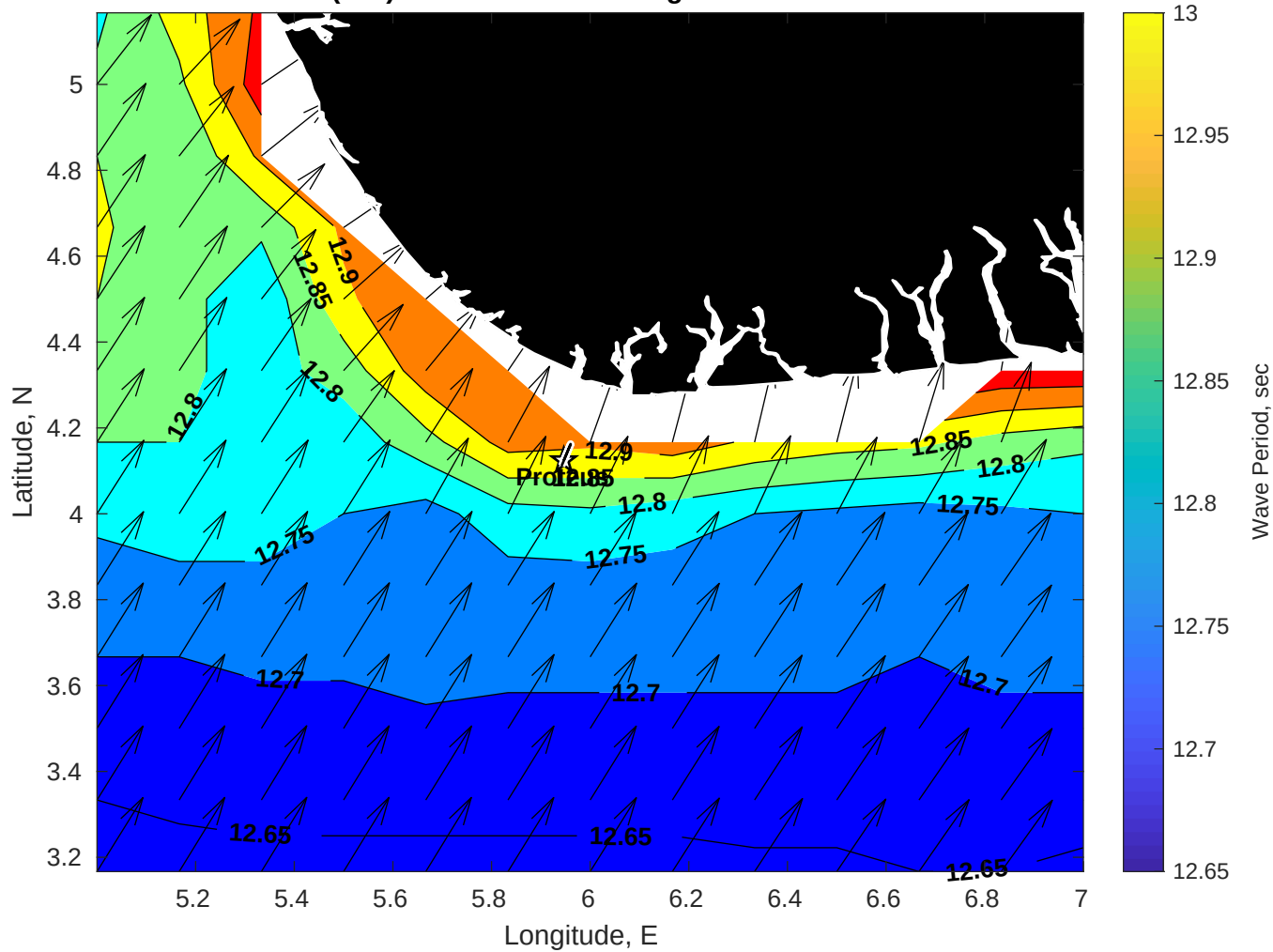
Wave Period (sec) for Proteus at 01-Aug-2025 21:00:00
