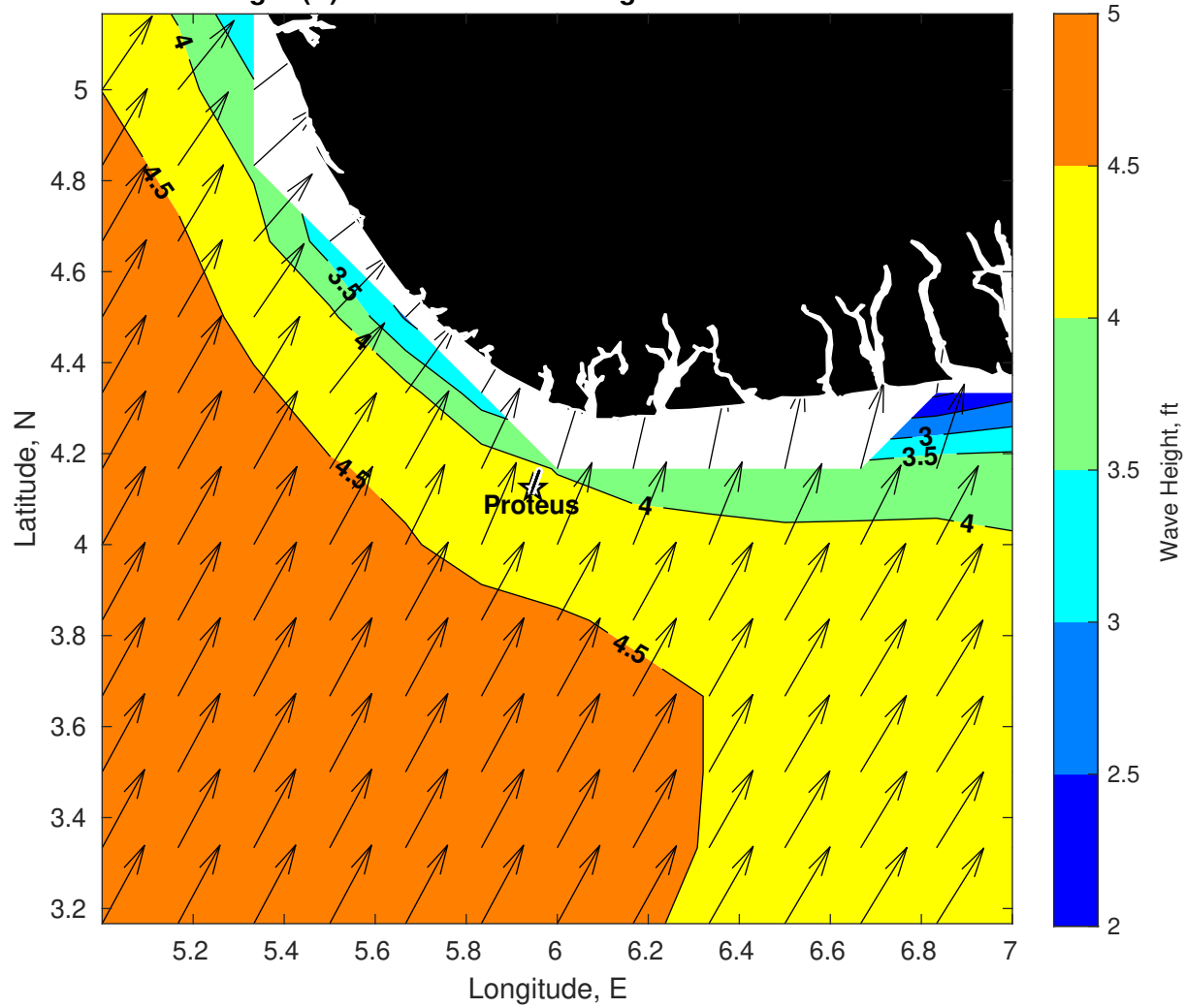
Wave Height (ft) for Proteus at 01-Aug-2025 21:00:00
