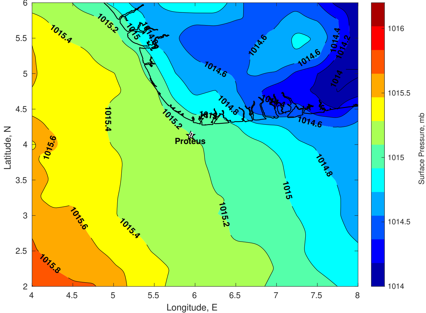
Surface Pressure (mb) for Proteus at 02-Aug-2025 12:00:00
