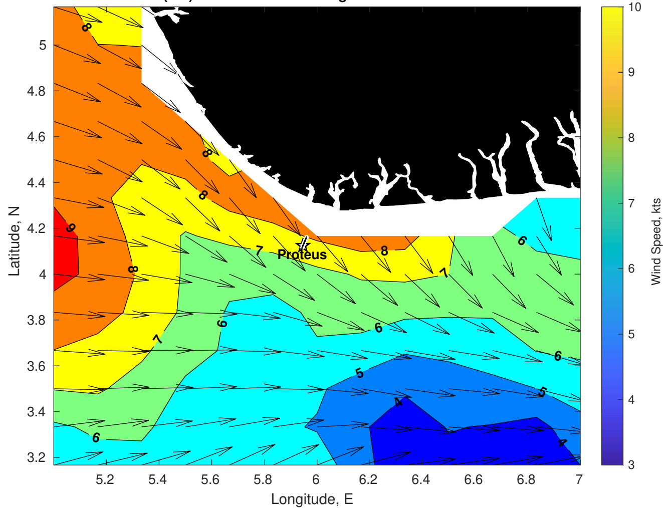
Winds (kts) for Proteus at 01-Aug-2025 21:00:00
