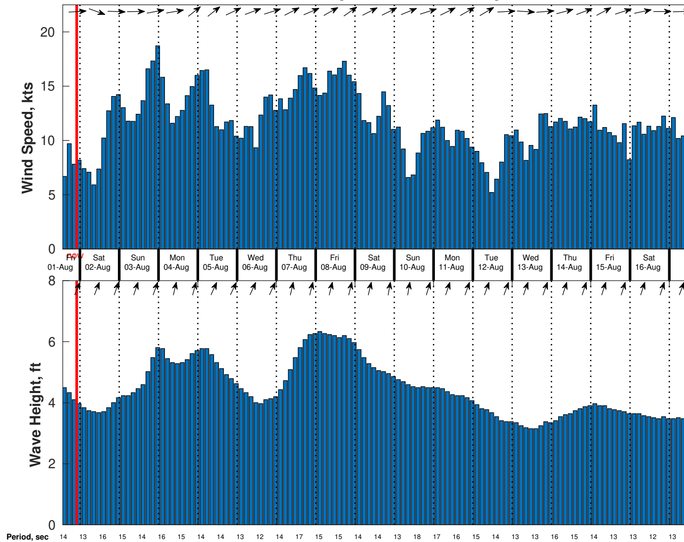
Wind & Wave Forecast for Proteus from 01-Aug-2025 13:00:00 to 17-Aug-2025 13:00:00
