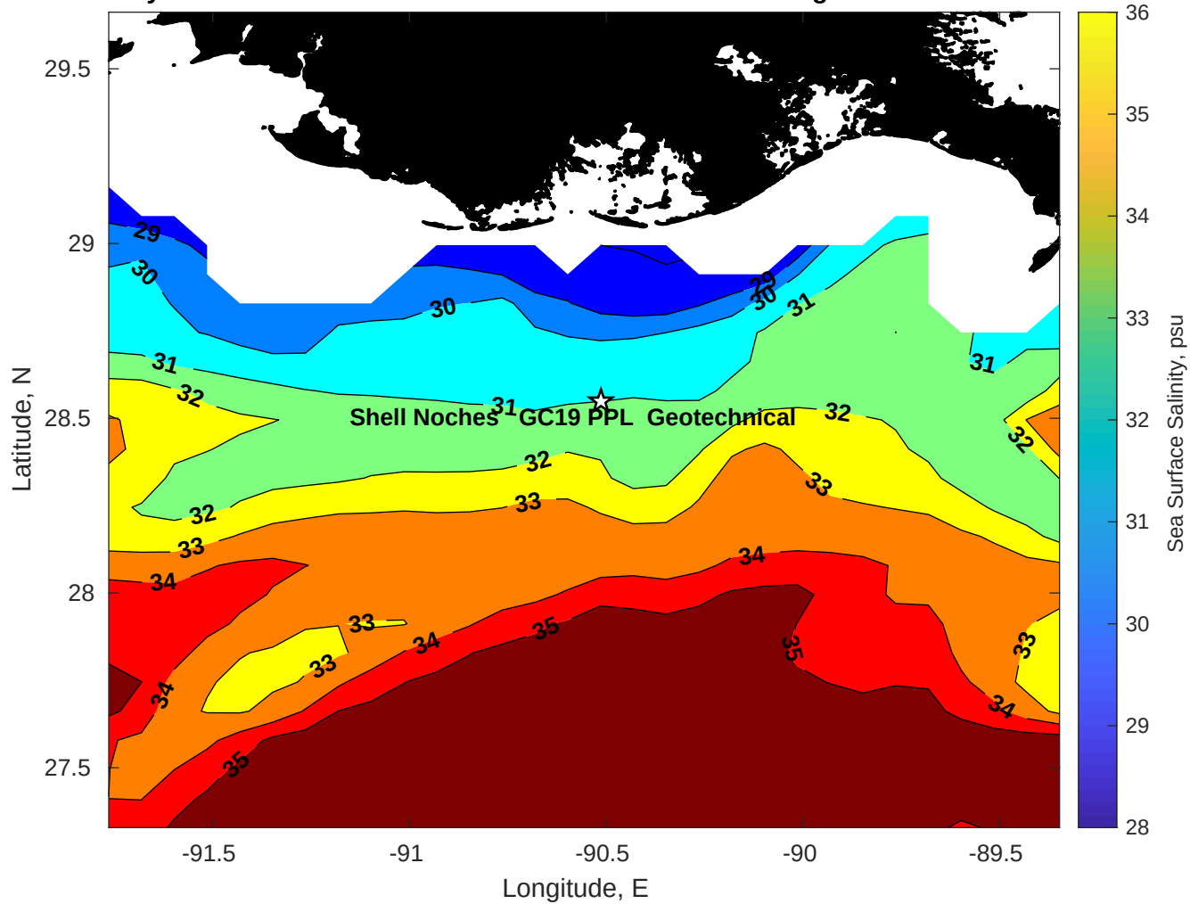
Surface Salinity for Shell Noches GC19 PPL Geotechnical at 01-Aug-2025 00:00:00
