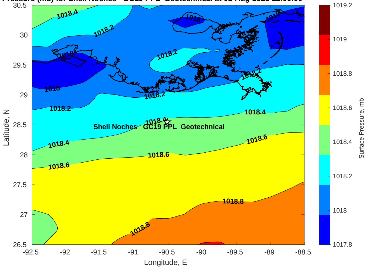
Surface Pressure (mb) for Shell Noches GC19 PPL Geotechnical at 01-Aug-2025 12:00:00
