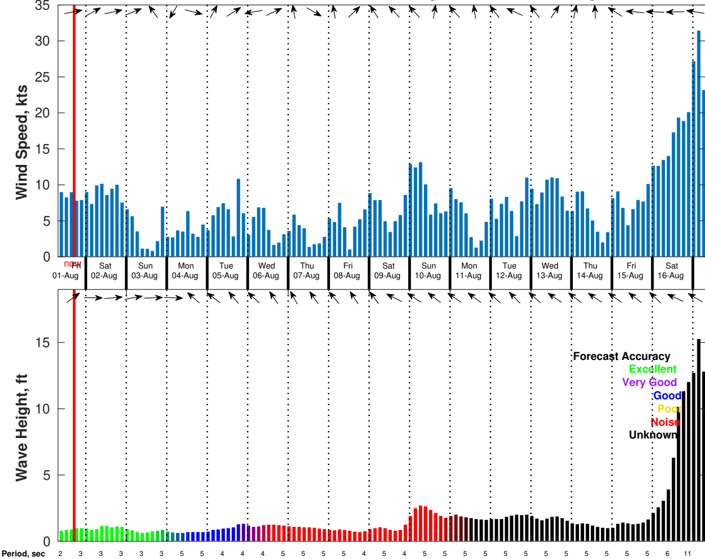
Wind & Wave Forecast for Shell Noches GC19 PPL Geotechnical from 01-Aug-2025 08:00:00 to 17-Aug-2025 08:00:00
