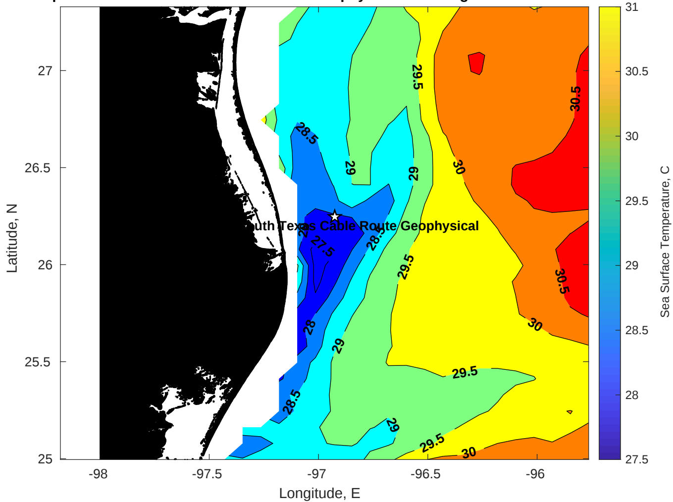
SST for Tampnet P2378 South Texas Cable Route Geophysical at 01-Aug-2025 00:00:00
