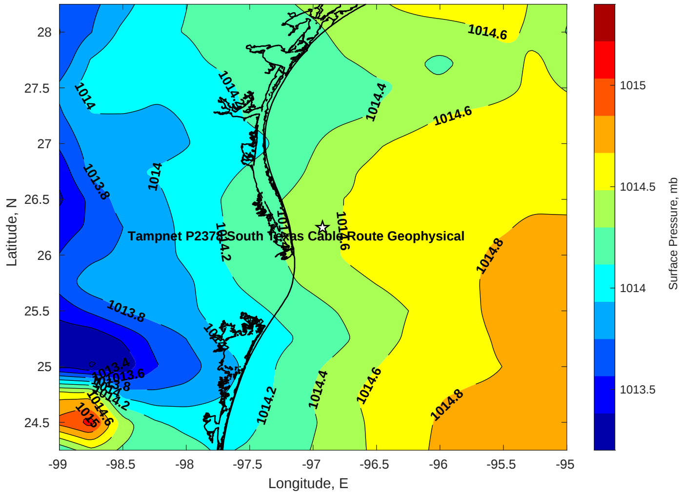
Pressure (mb) for Tampnet P2378 South Texas Cable Route Geophysical at 03-Aug-2025 12:00:00
