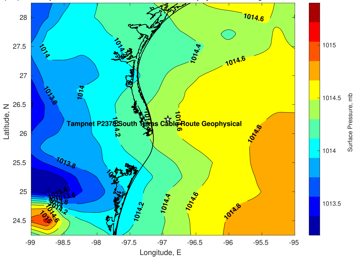
Pressure (mb) for Tampnet P2378 South Texas Cable Route Geophysical at 03-Aug-2025 12:00:00
