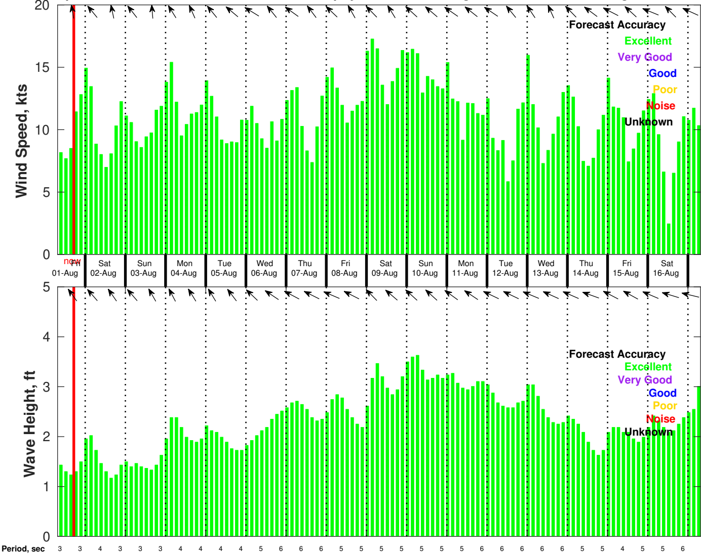
Wind & Wave Forecast for Tampnet P2378 South Texas Cable Route Geophysical from 01-Aug-2025 08:00:00 to 17-Aug-2025 08:00:00
