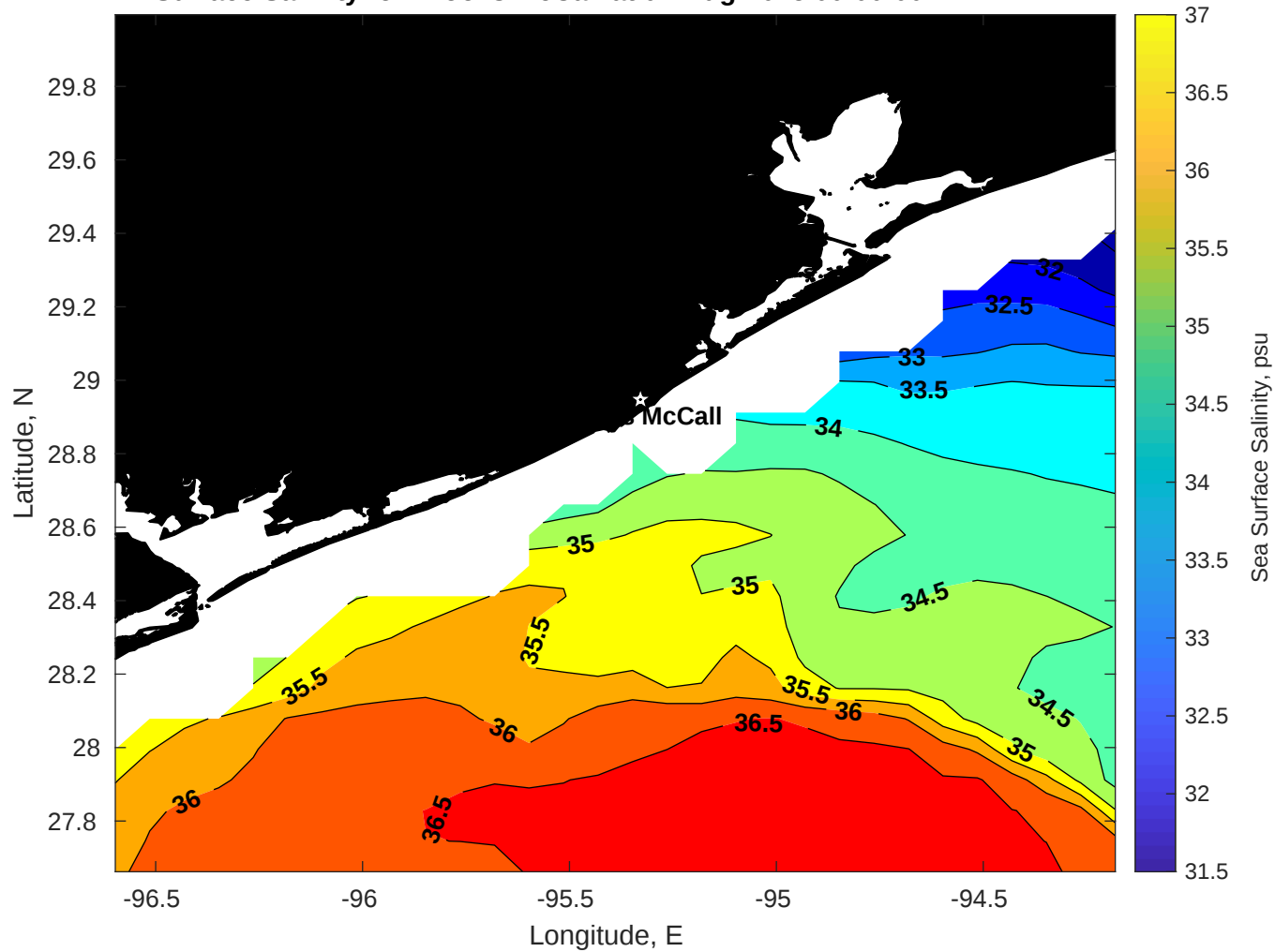
Surface Salinity for Brooks McCall at 02-Aug-2025 00:00:00
