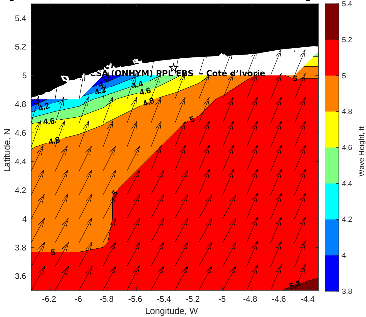
Wave Height (ft) for CSA (ONHYM) PPL EBS - Cote d'Ivoire at 03-Aug-2025 09:00:00
