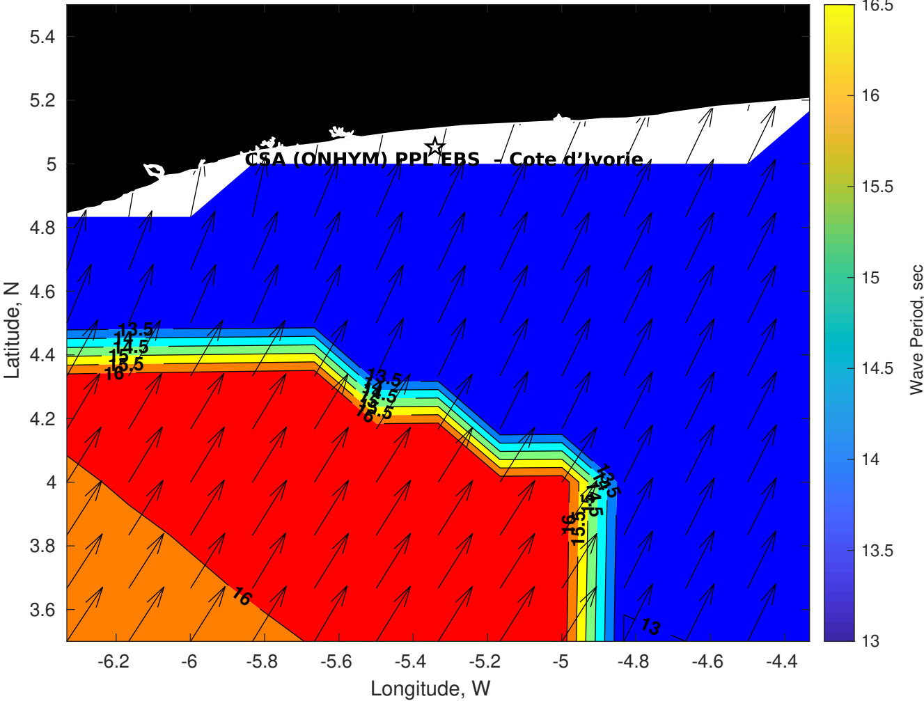
Wave Period (sec) for CSA (ONHYM) PPL EBS - Cote d'Ivoire at 03-Aug-2025 09:00:00
