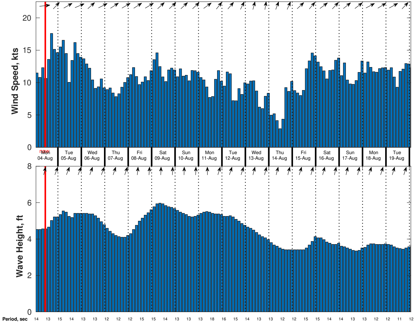
Wind & Wave Forecast for CSA (ONHYM) PPL EBS - Cote d'Ivoire from 03-Aug-2025 01:00:00 to 19-Aug-2025 01:00:00
