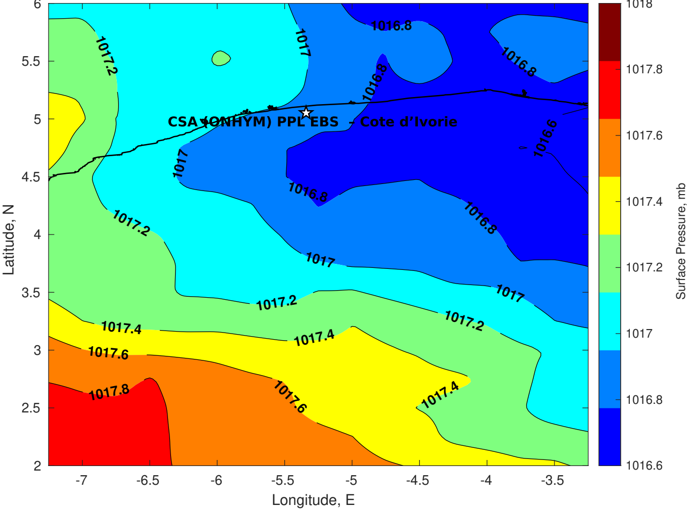
Surface Pressure (mb) for CSA (ONHYM) PPL EBS - Cote d'Ivoire at 05-Aug-2025 00:00:00
