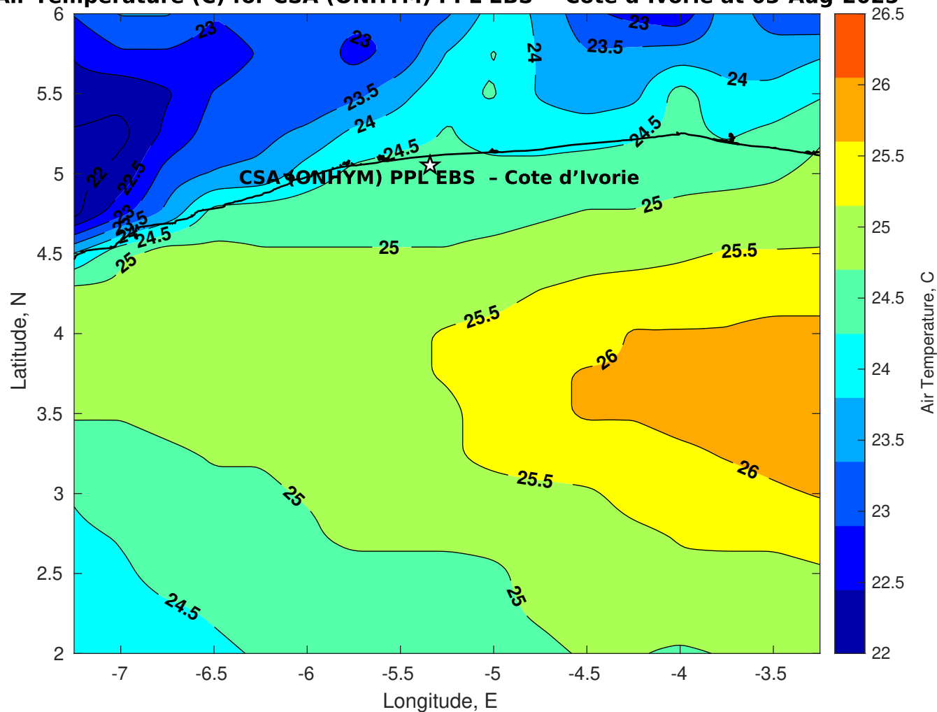
Air Temperature (C) for CSA (ONHYM) PPL EBS - Cote d'Ivoire at 03-Aug-2025
