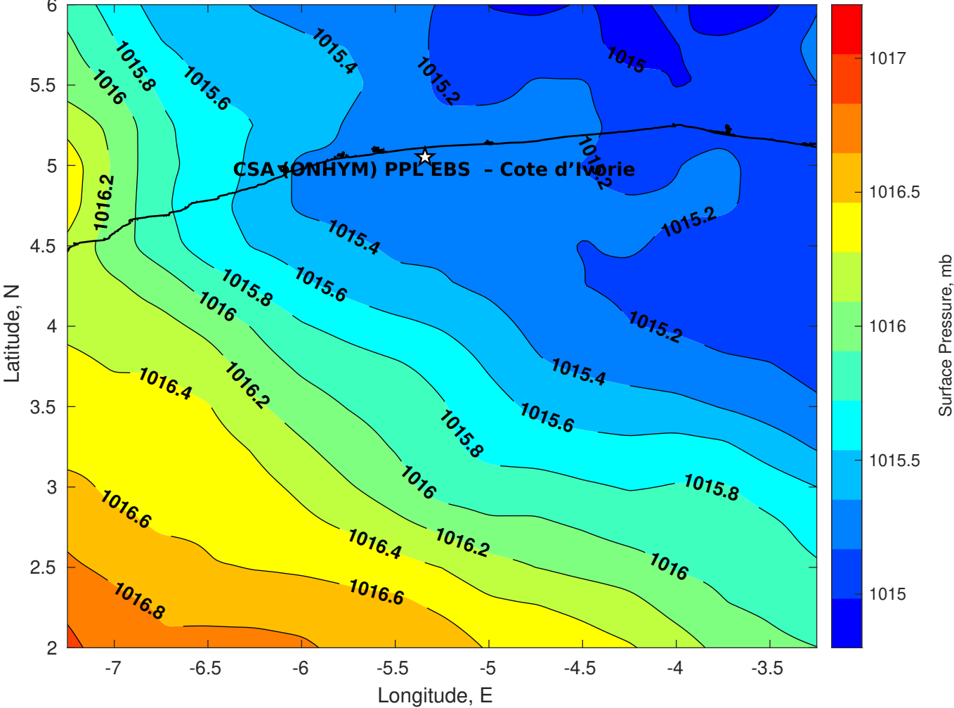
Surface Pressure (mb) for CSA (ONHYM) PPL EBS - Cote d'Ivoire at 04-Aug-2025 00:00:00
