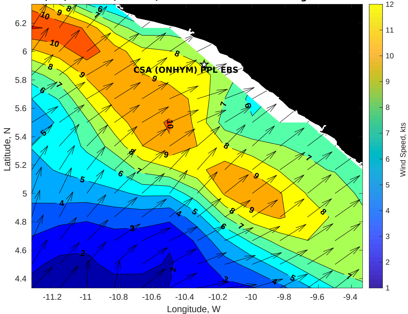
Winds (kts) for CSA (ONHYM) PPL EBS - Liberia at 03-Aug-2025 09:00:00
