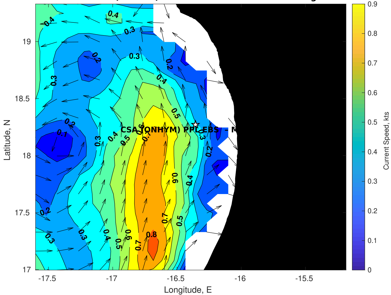
Surface Currents for CSA (ONHYM) PPL EBS - Mauritania at 01-Aug-2025 00:00:00
