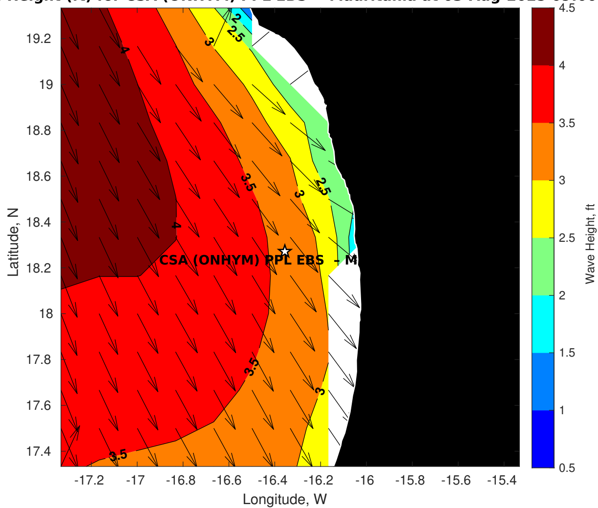
Wave Height (ft) for CSA (ONHYM) PPL EBS - Mauritania at 03-Aug-2025 09:00:00
