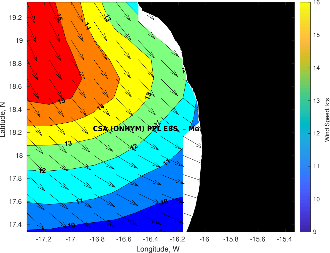
Winds (kts) for CSA (ONHYM) PPL EBS - Mauritania at 03-Aug-2025 09:00:00
