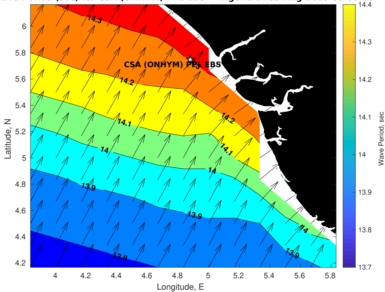
Wave Period (sec) for CSA (ONHYM) PPL EBS - Nigeria at 03-Aug-2025 09:00:00
