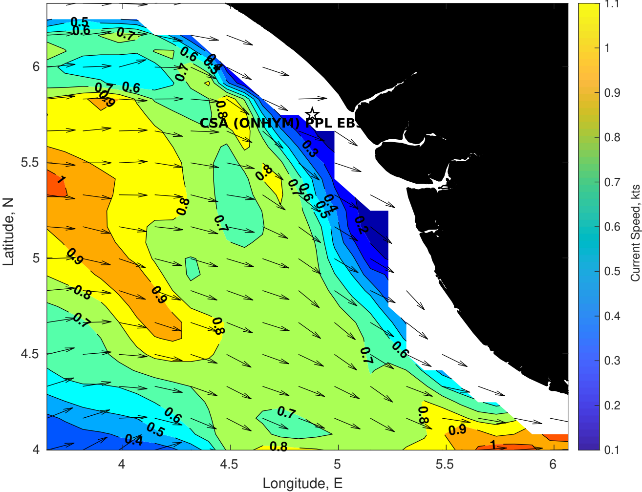
Surface Currents for CSA (ONHYM) PPL EBS - Nigeria at 01-Aug-2025 00:00:00
