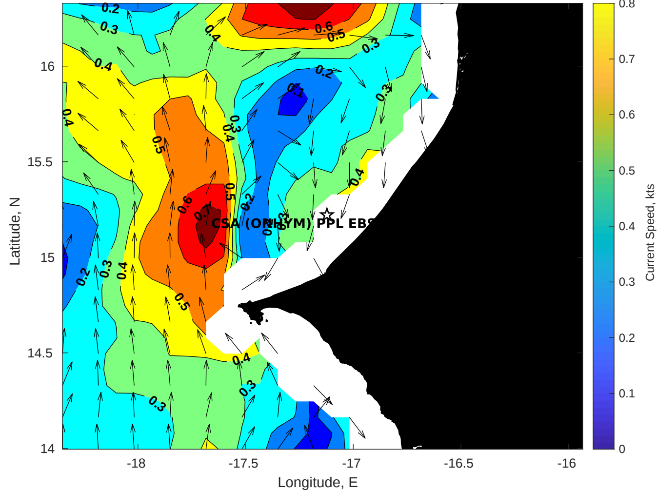
Surface Currents for CSA (ONHYM) PPL EBS - Senegal at 01-Aug-2025 00:00:00
