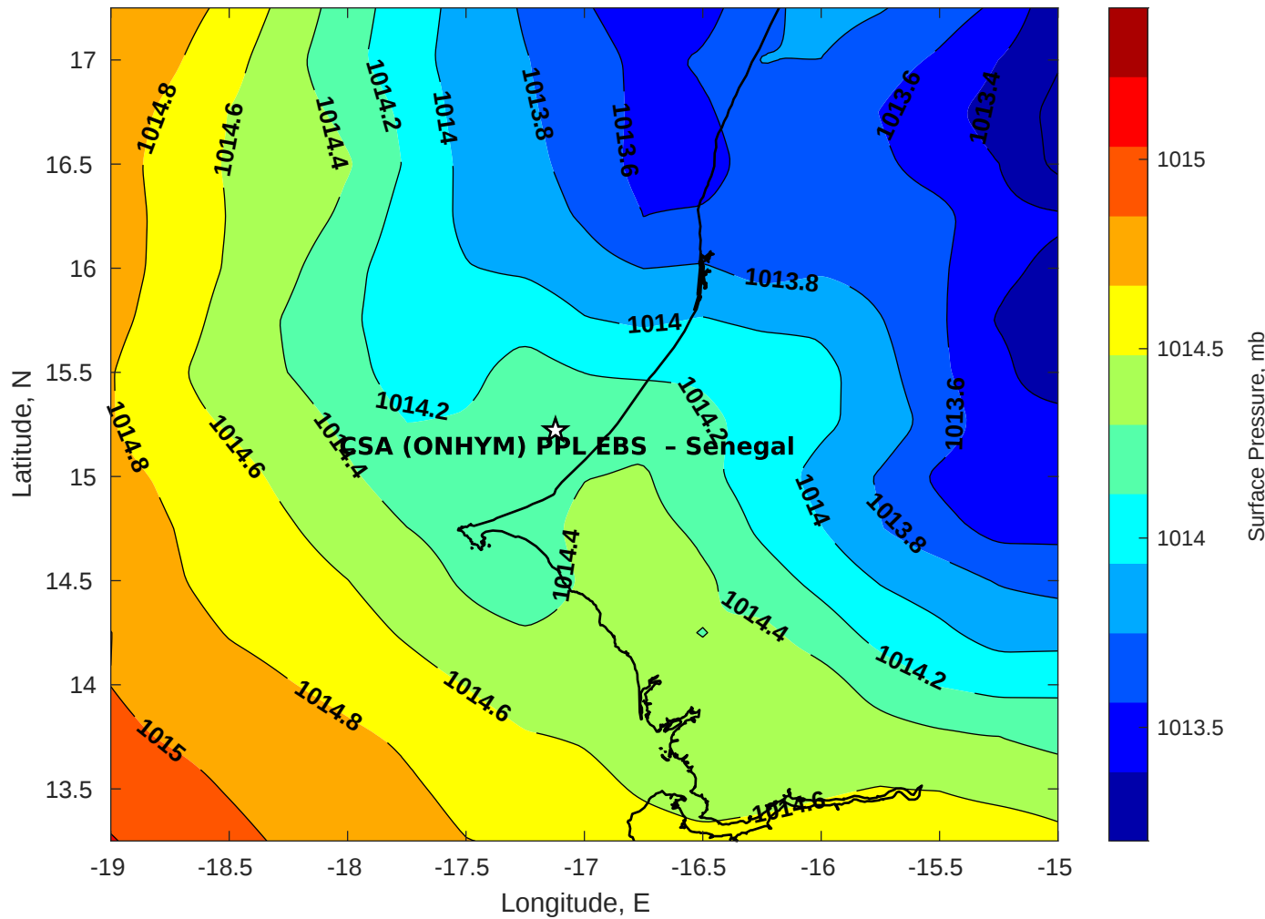
Surface Pressure (mb) for CSA (ONHYM) PPL EBS - Senegal at 05-Aug-2025 00:00:00
