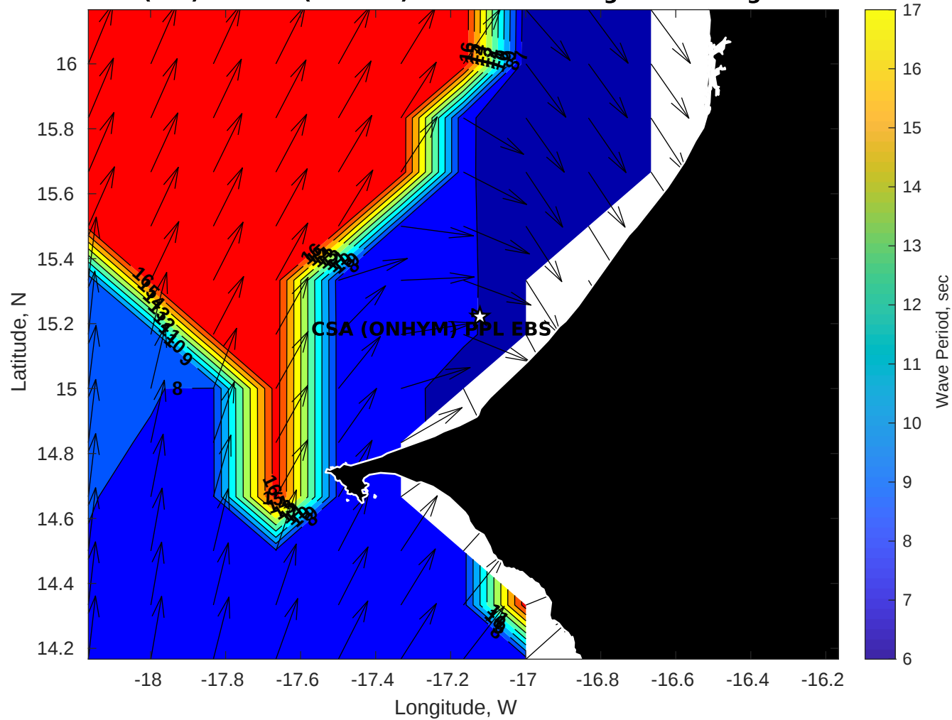
Wave Period (sec) for CSA (ONHYM) PPL EBS - Senegal at 03-Aug-2025 09:00:00
