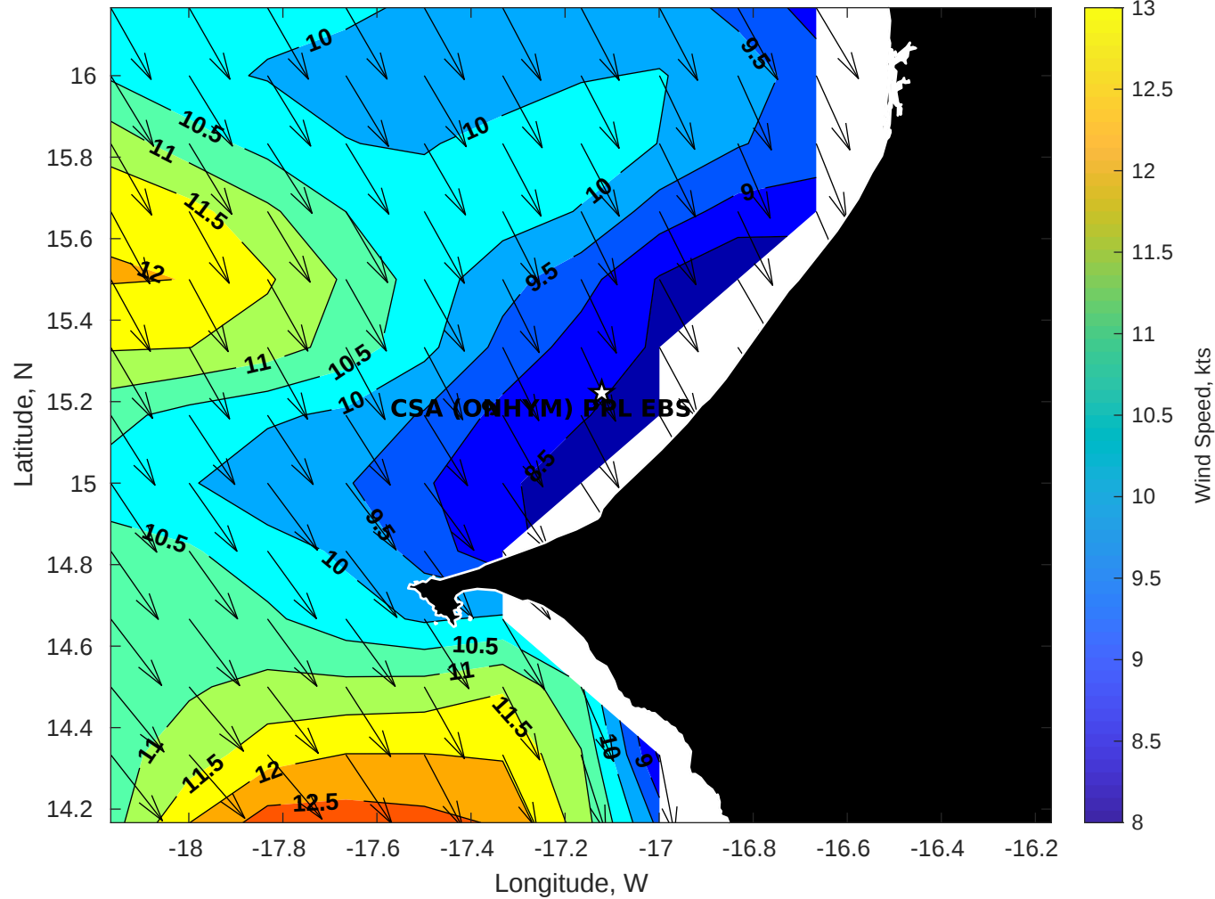
Winds (kts) for CSA (ONHYM) PPL EBS - Senegal at 03-Aug-2025 09:00:00
