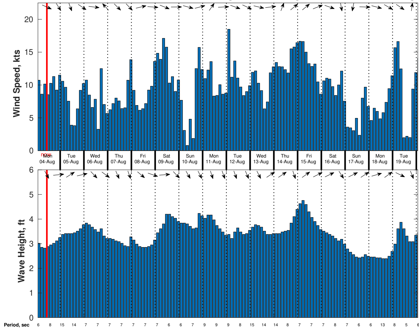
Wind & Wave Forecast for CSA (ONHYM) PPL EBS - Senegal from 03-Aug-2025 01:00:00 to 19-Aug-2025 01:00:00
