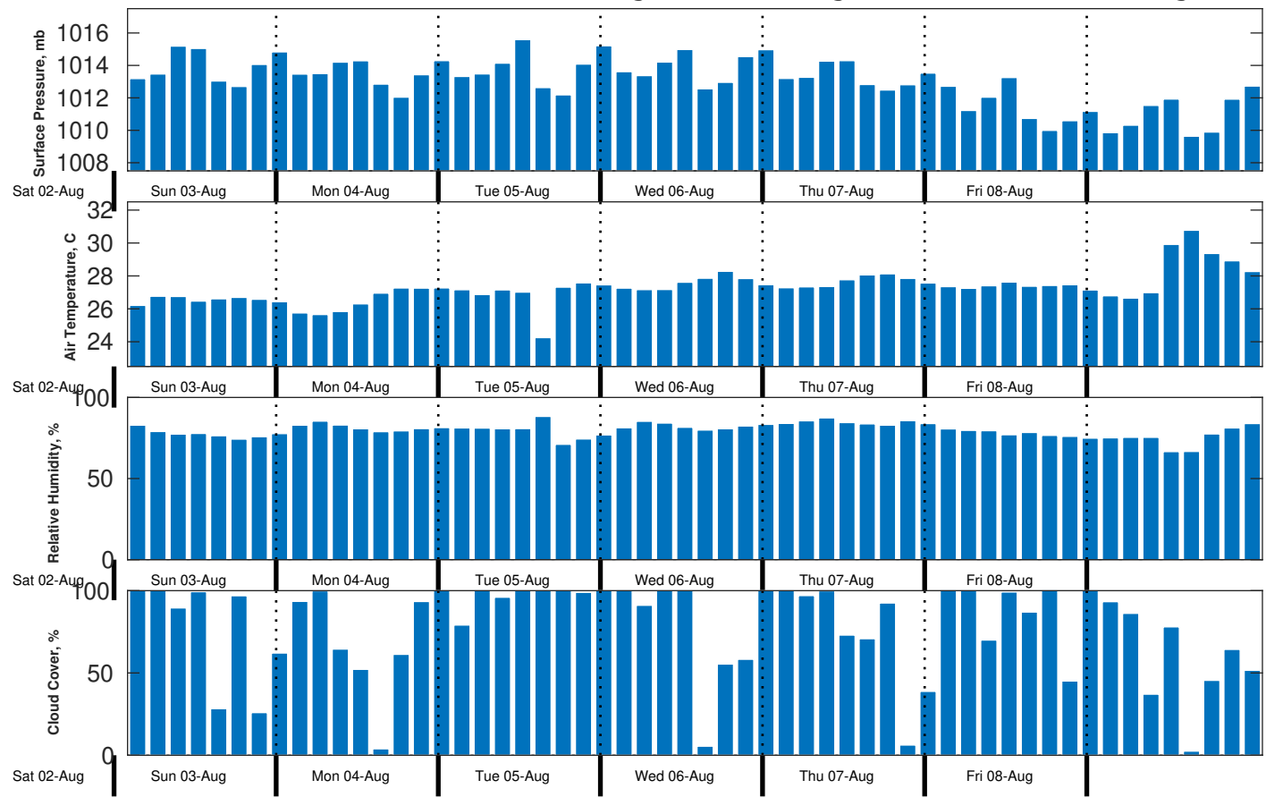
Met Forecast for CSA (ONHYM) PPL EBS - Senegal from 03-Aug-2025 00:00:00 to 10-Aug-2025 00:00:00
