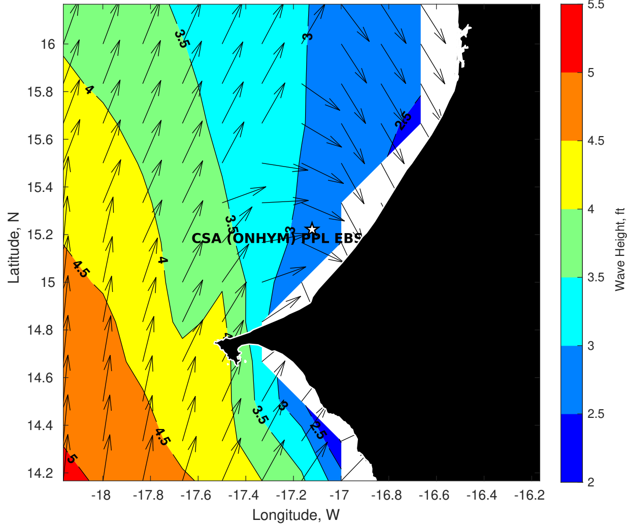
Wave Height (ft) for CSA (ONHYM) PPL EBS - Senegal at 03-Aug-2025 09:00:00
