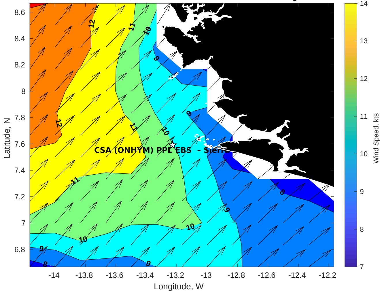
Winds (kts) for CSA (ONHYM) PPL EBS - Sierra Leone at 03-Aug-2025 09:00:00
