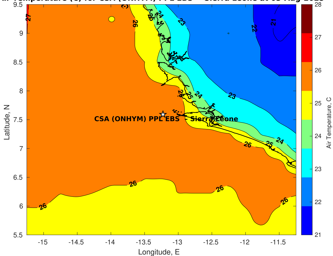
Air Temperature (C) for CSA (ONHYM) PPL EBS - Sierra Leone at 03-Aug-2025
