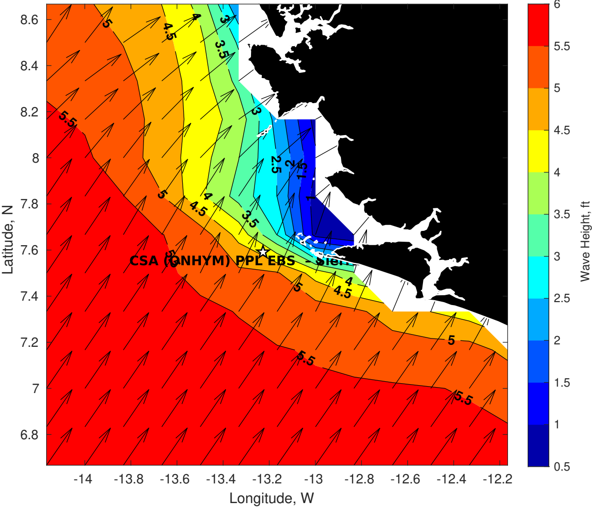
Wave Height (ft) for CSA (ONHYM) PPL EBS - Sierra Leone at 03-Aug-2025 09:00:00
