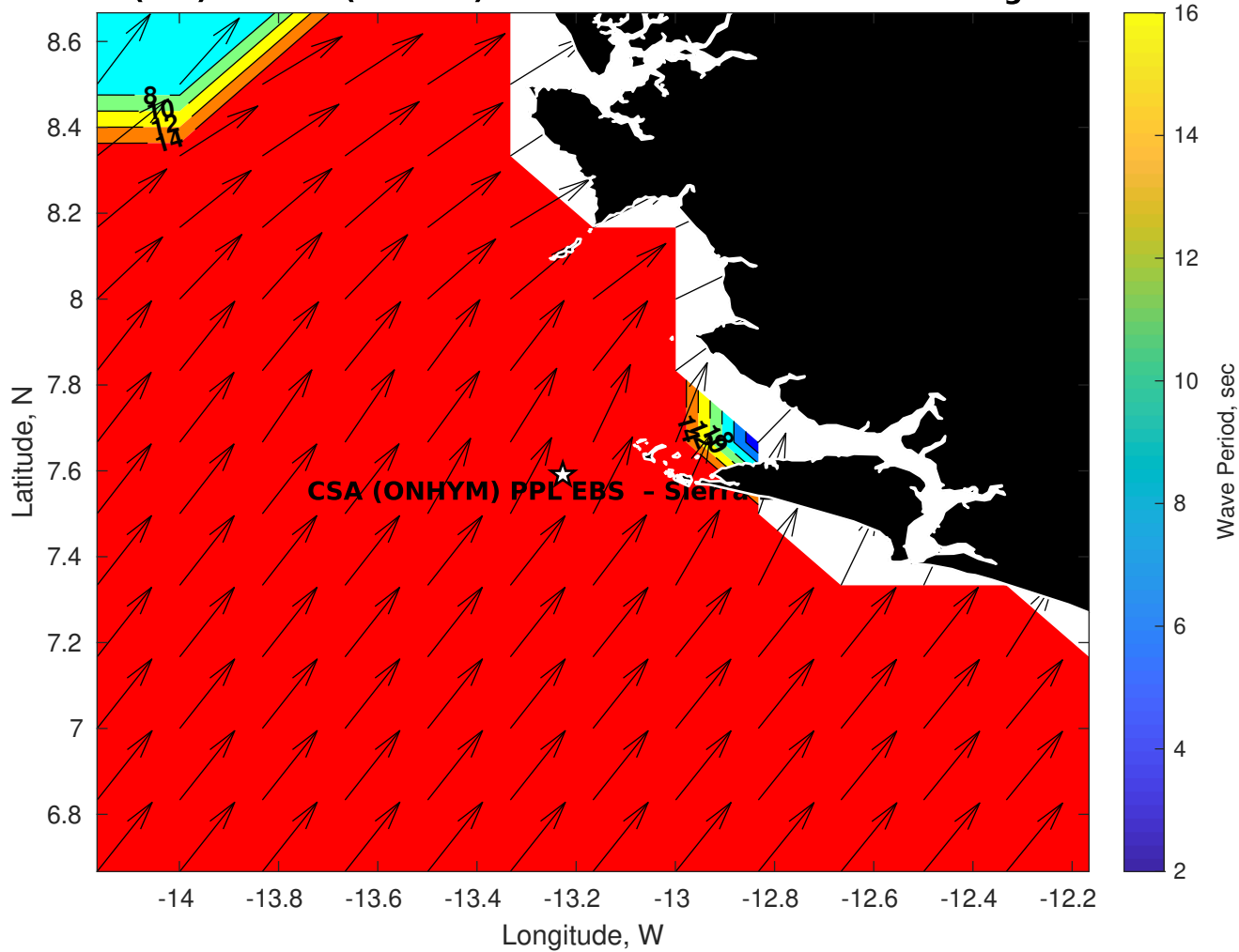
Wave Period (sec) for CSA (ONHYM) PPL EBS - Sierra Leone at 03-Aug-2025 09:00:00
