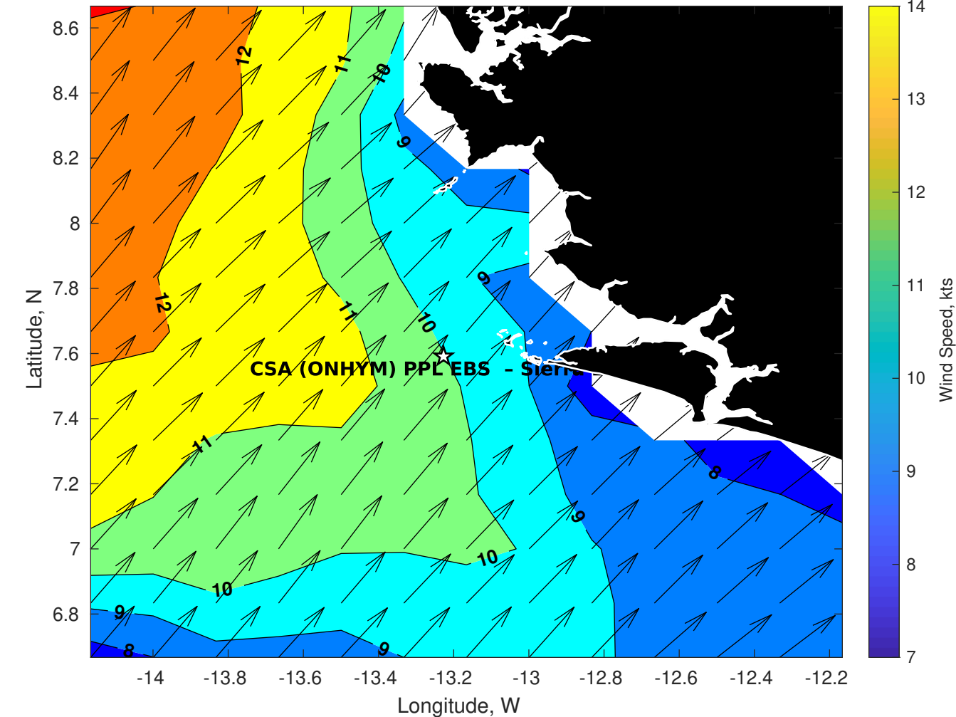
Winds (kts) for CSA (ONHYM) PPL EBS - Sierra Leone at 03-Aug-2025 09:00:00
