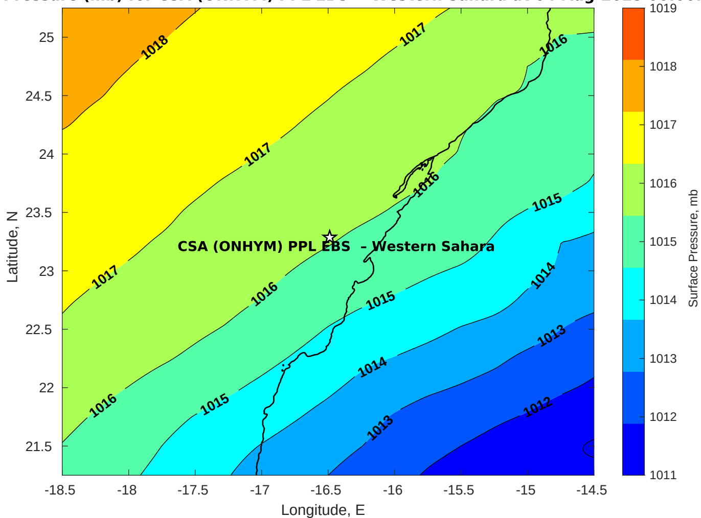
Surface Pressure (mb) for CSA (ONHYM) PPL EBS - Western Sahara at 04-Aug-2025 00:00:00
