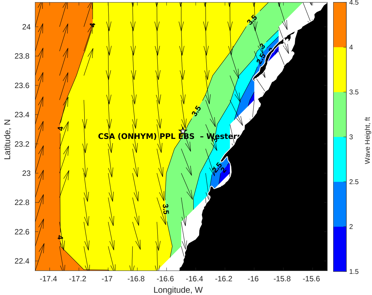
Wave Height (ft) for CSA (ONHYM) PPL EBS - Western Sahara at 03-Aug-2025 09:00:00
