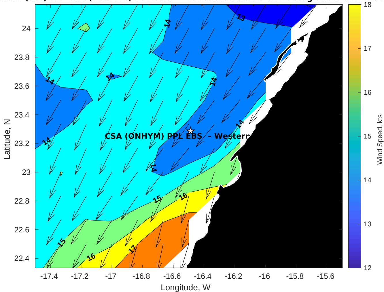
Winds (kts) for CSA (ONHYM) PPL EBS - Western Sahara at 03-Aug-2025 09:00:00
