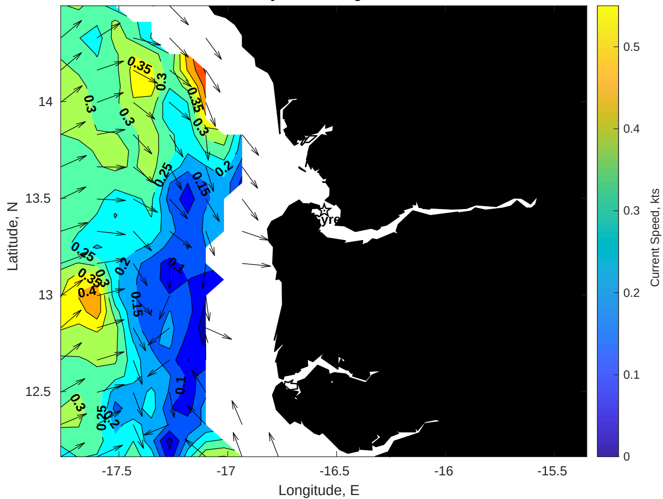
Surface Currents for Gyre at 02-Aug-2025 00:00:00
