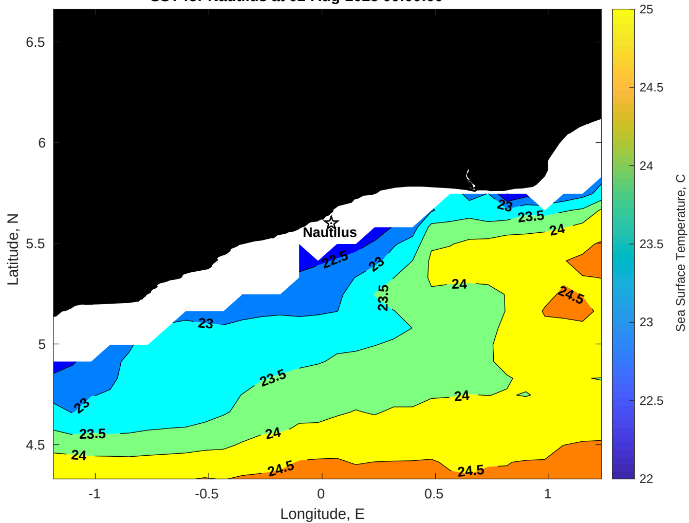
SST for Nautilus at 02-Aug-2025 00:00:00
