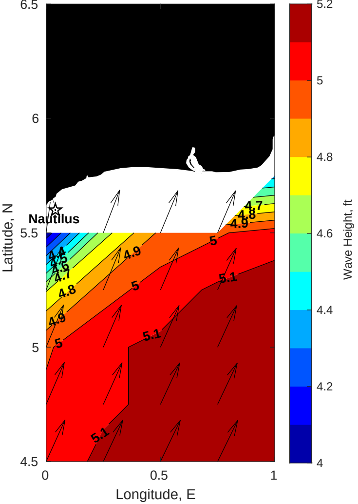
Wave Height (ft) for Nautilus at 03-Aug-2025 09:00:00
