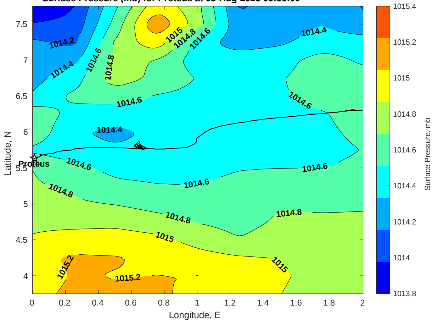
Surface Pressure (mb) for Proteus at 03-Aug-2025 00:00:00
