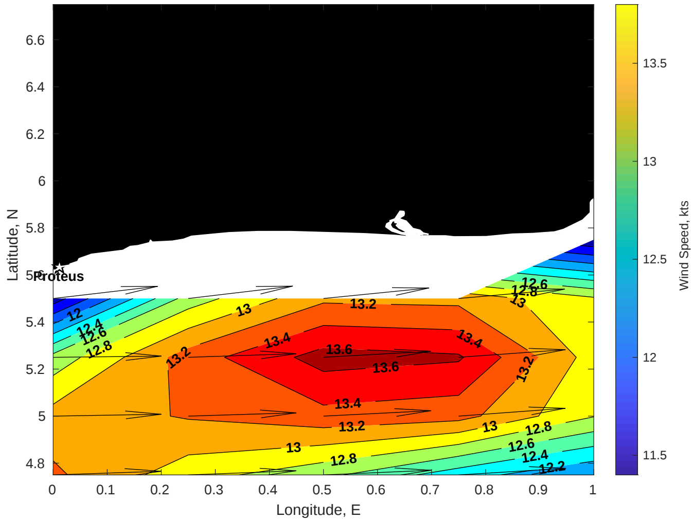
Winds (kts) for Proteus at 03-Aug-2025 09:00:00
