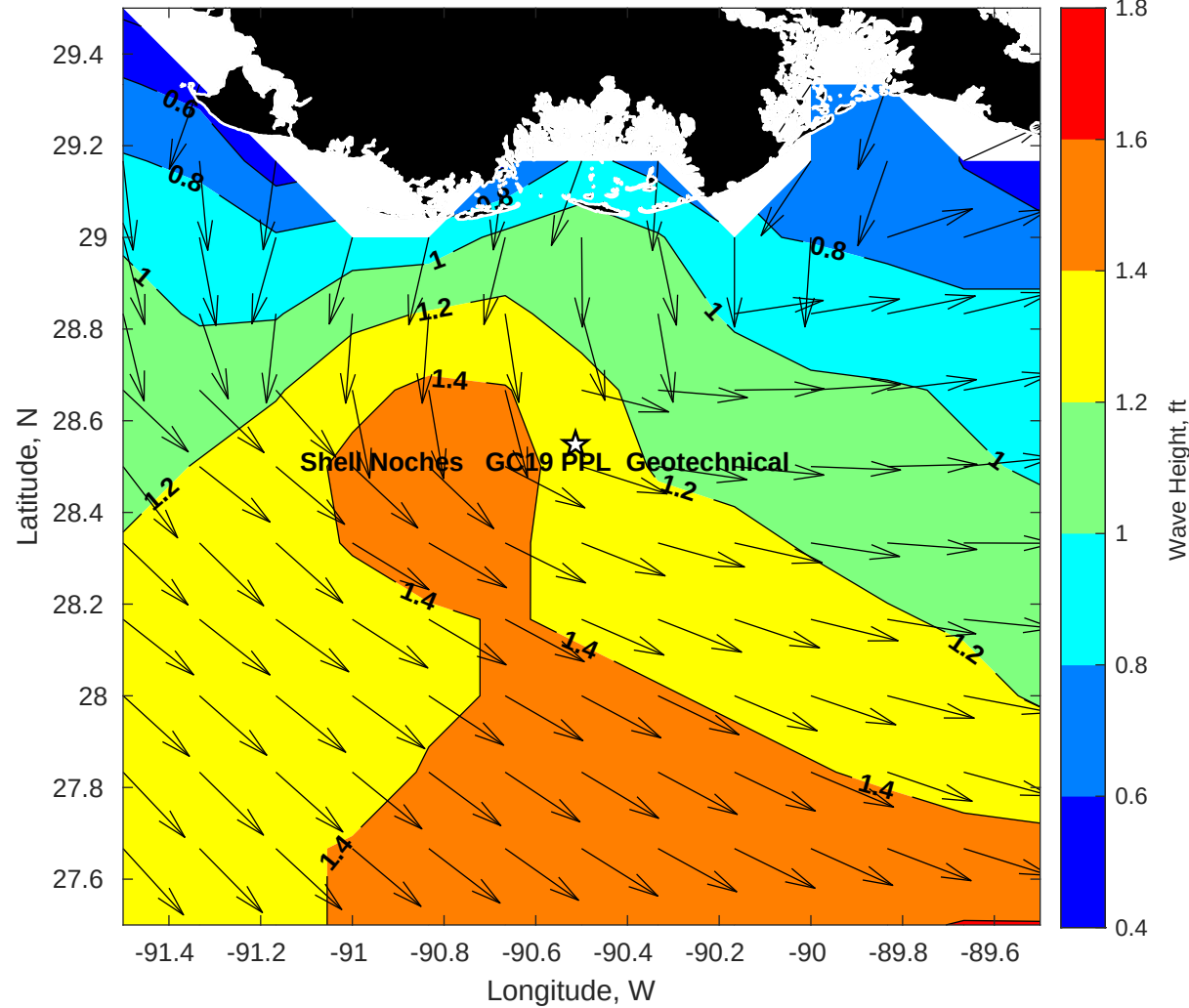
Wave Height (ft) for Shell Noches GC19 PPL Geotechnical at 03-Aug-2025 09:00:00
