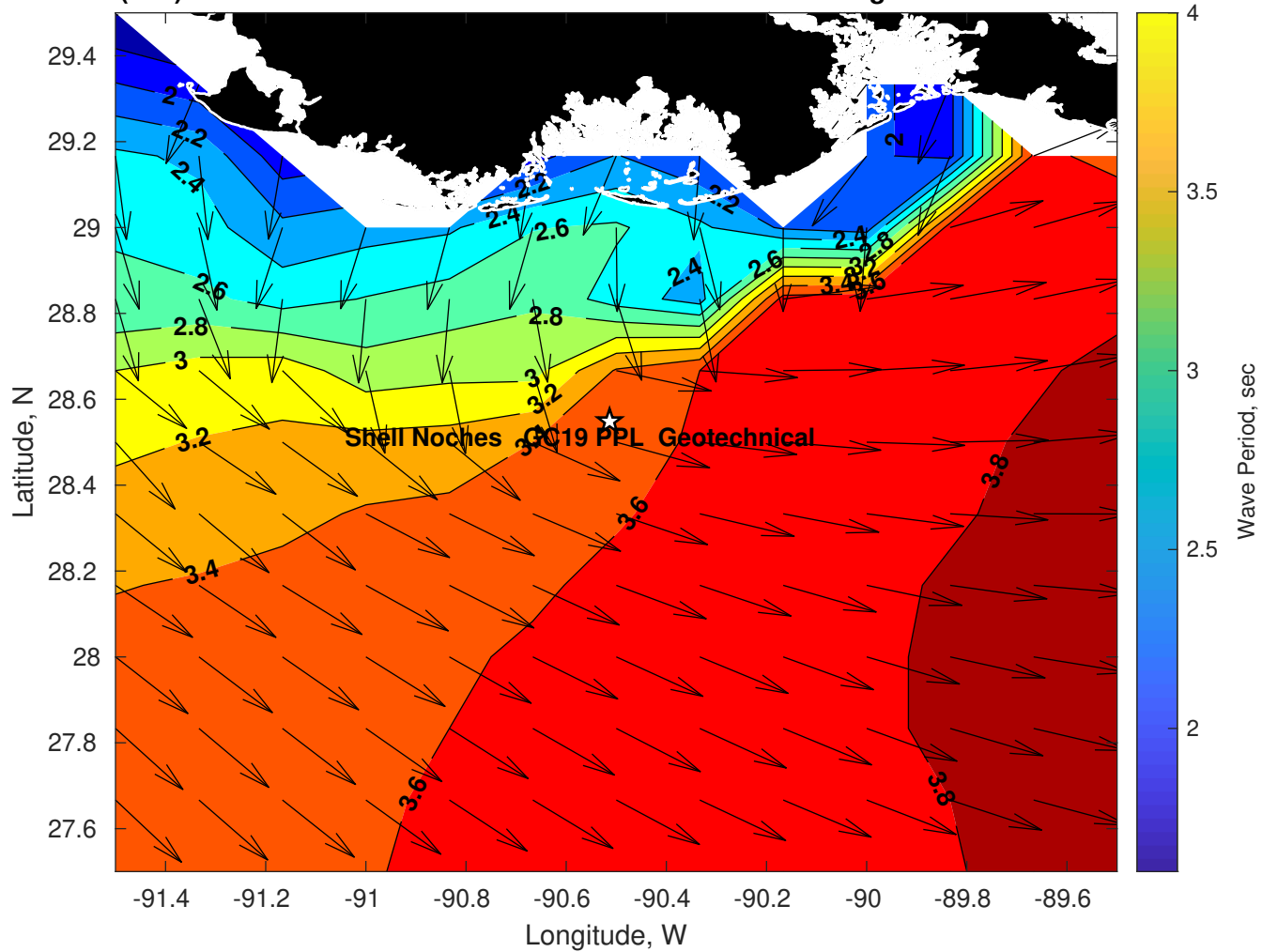
Wave Period (sec) for Shell Noches GC19 PPL Geotechnical at 03-Aug-2025 09:00:00
