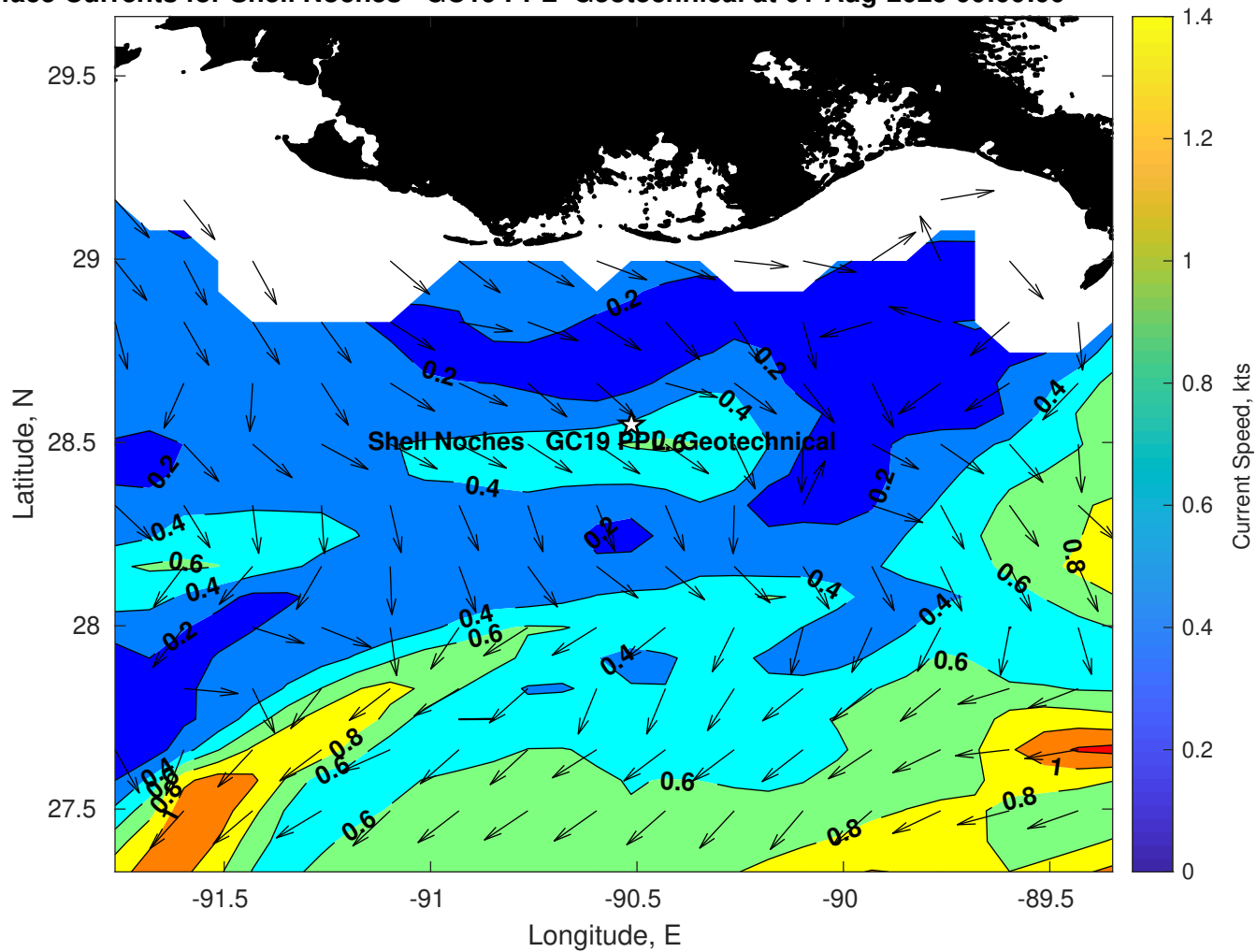
Surface Currents for Shell Noches GC19 PPL Geotechnical at 01-Aug-2025 00:00:00
