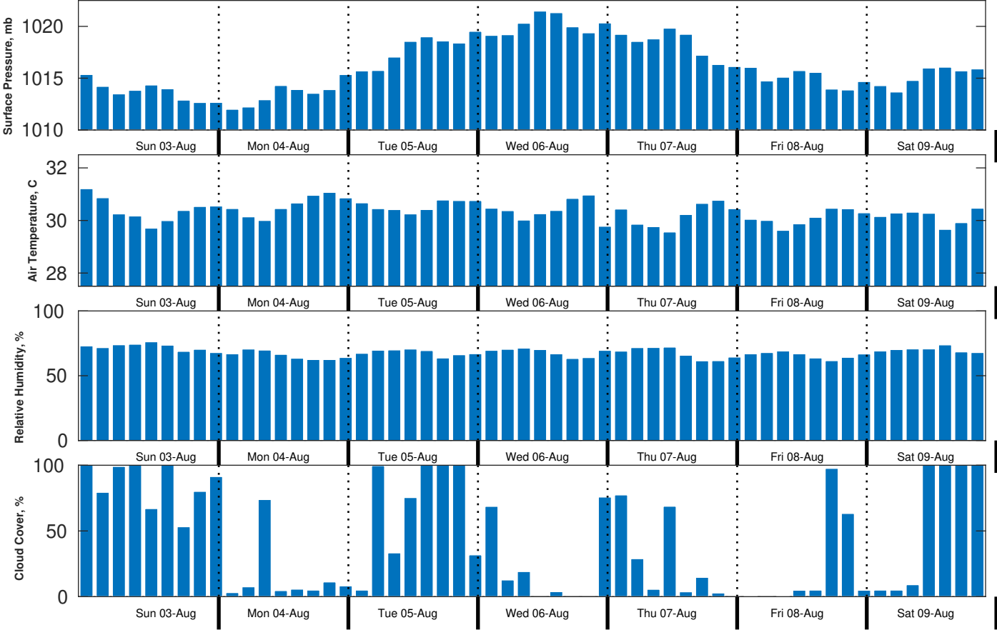
Met Forecast for Shell Noches GC19 PPL Geotechnical from 03-Aug-2025 00:00:00 to 10-Aug-2025 00:00:00
