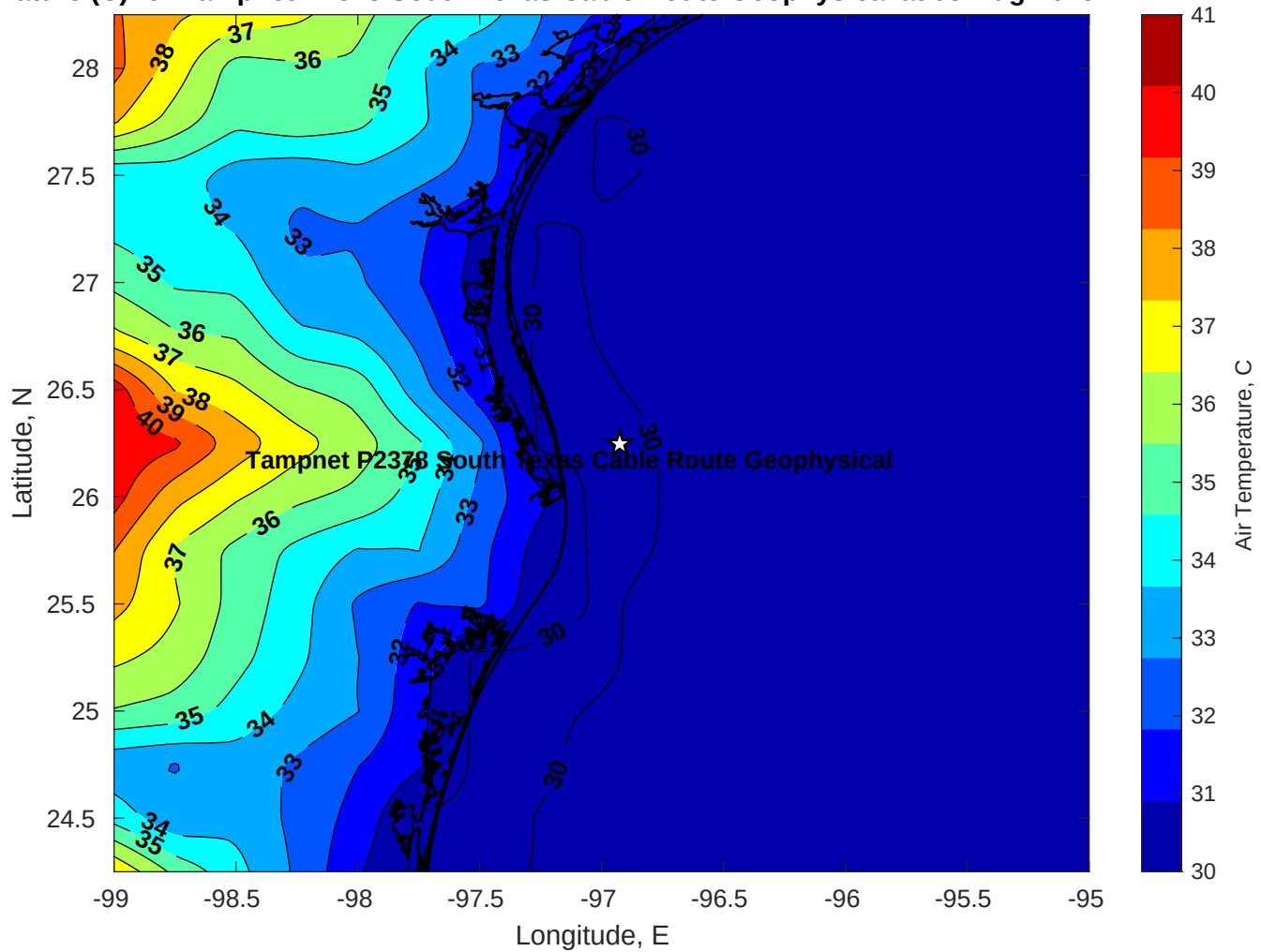
Air Temperature (C) for Tampnet P2378 South Texas Cable Route Geophysical at 03-Aug-2025
