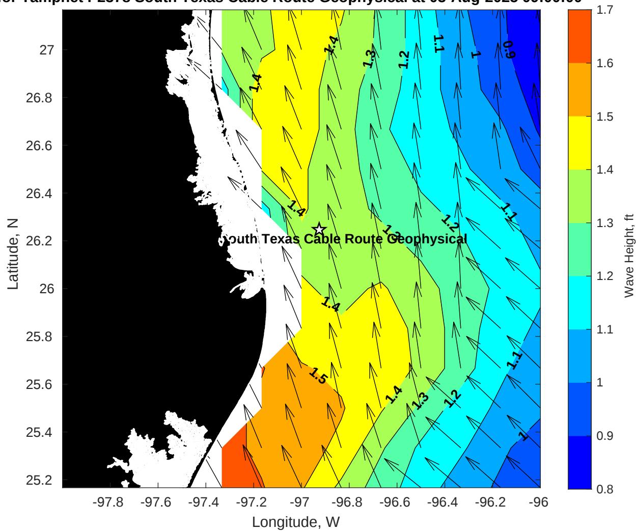
Wave Height (ft) for Tampnet P2378 South Texas Cable Route Geophysical at 03-Aug-2025 09:00:00
