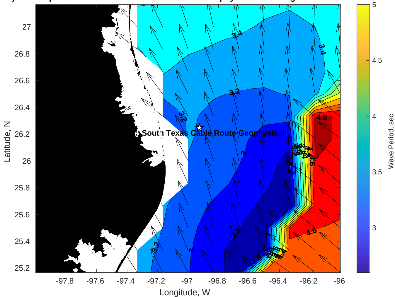
Period (sec) for Tampnet P2378 South Texas Cable Route Geophysical at 03-Aug-2025 09:00:00
