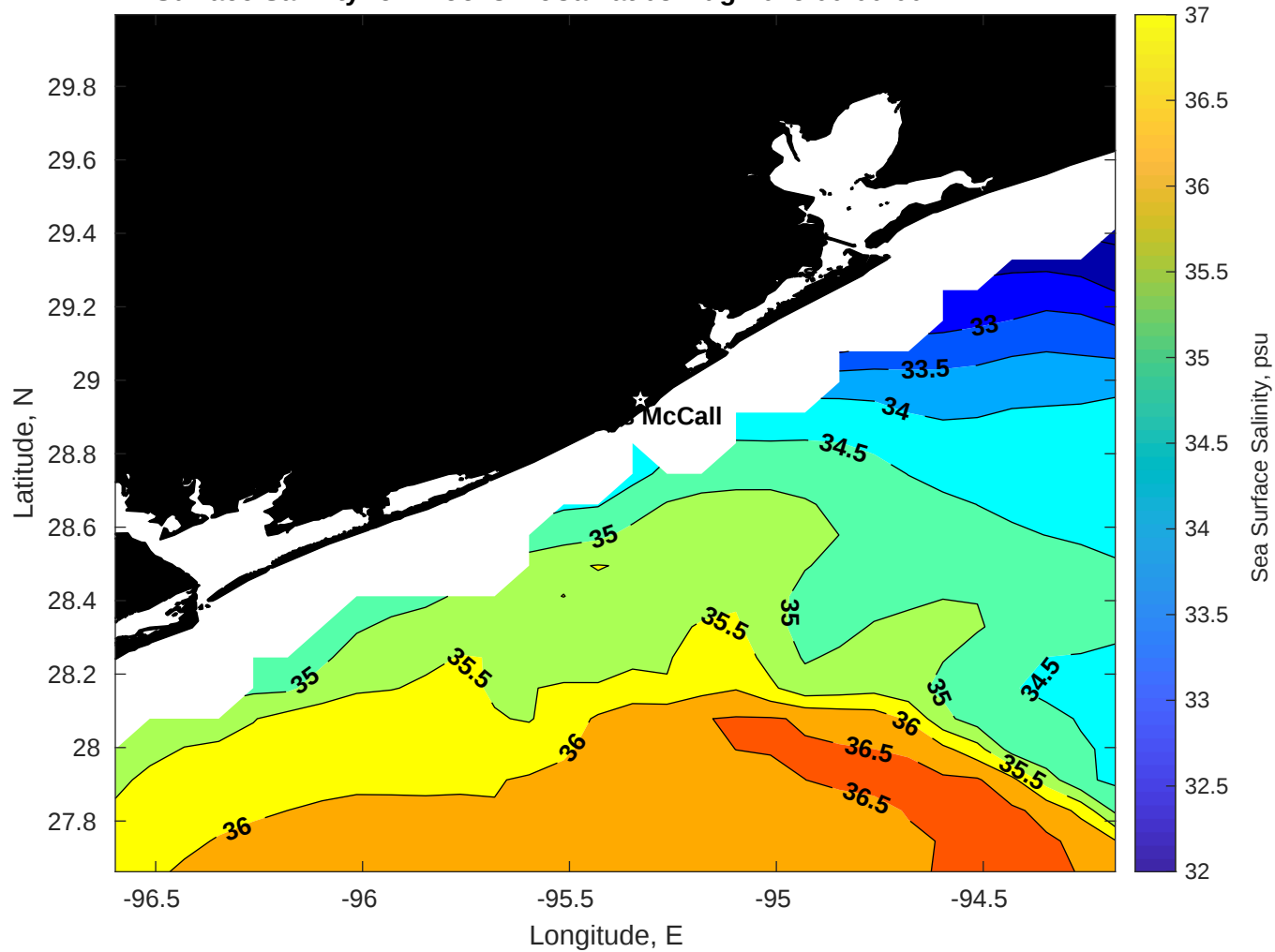
Surface Salinity for Brooks McCall at 03-Aug-2025 00:00:00
