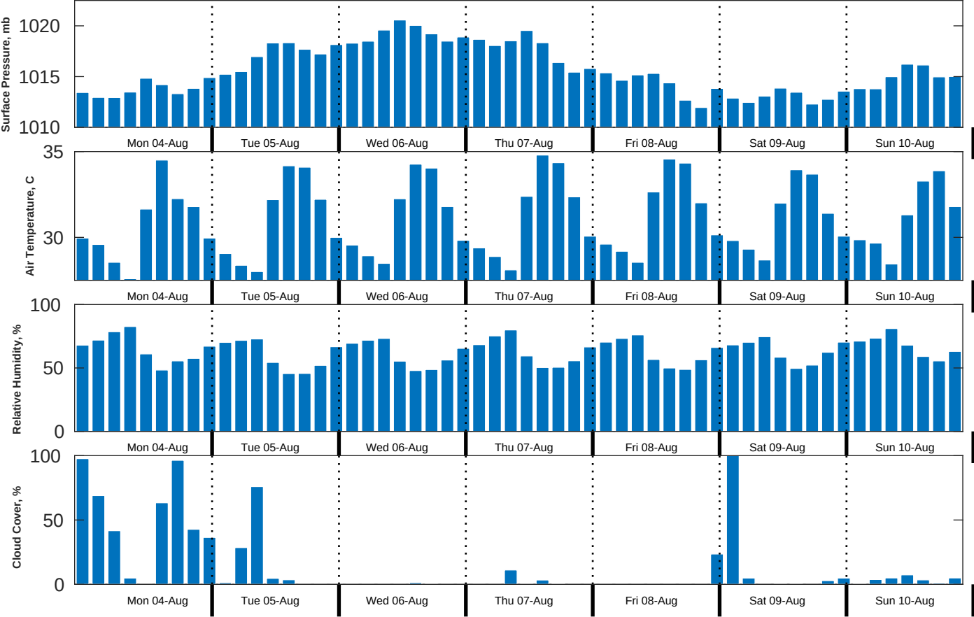
Met Forecast for Brooks McCall from 04-Aug-2025 00:00:00 to 11-Aug-2025 00:00:00
