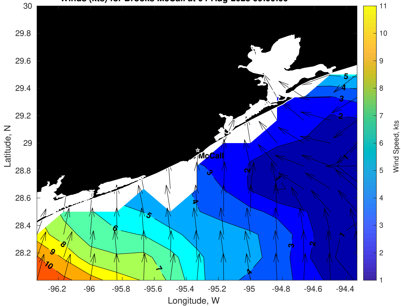
Winds (kts) for Brooks McCall at 04-Aug-2025 09:00:00
