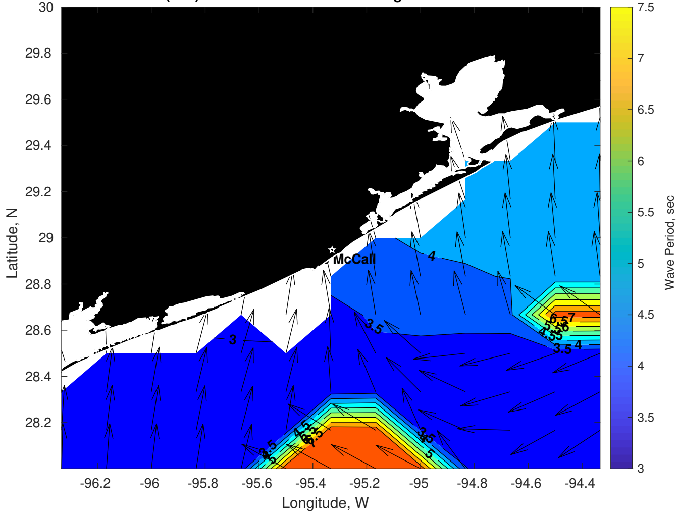
Wave Period (sec) for Brooks McCall at 04-Aug-2025 09:00:00
