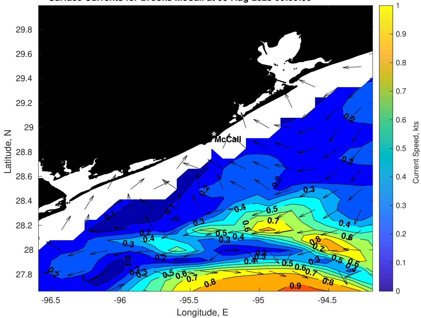
Surface Currents for Brooks McCall at 03-Aug-2025 00:00:00
