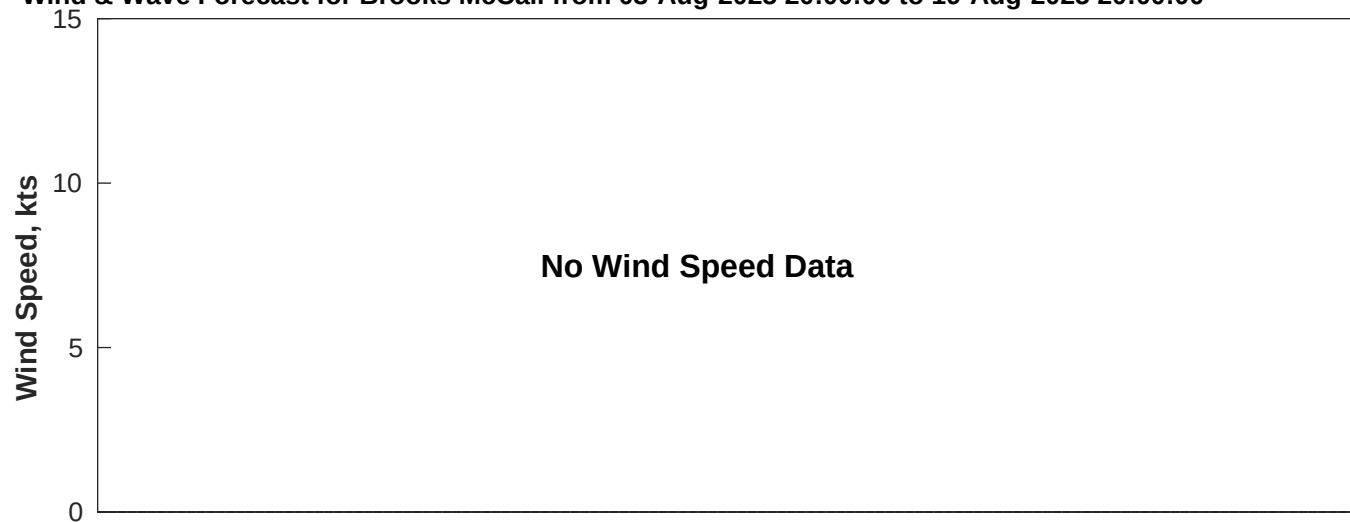
Wind & Wave Forecast for Brooks McCall from 03-Aug-2025 20:00:00 to 19-Aug-2025 20:00:00
