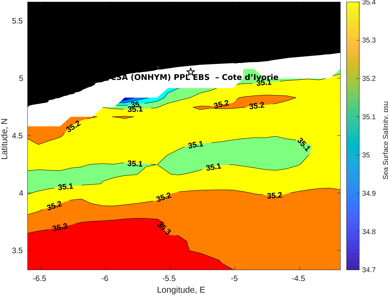
Surface Salinity for CSA (ONHYM) PPL EBS - Cote d'Ivoire at 03-Aug-2025 00:00:00
