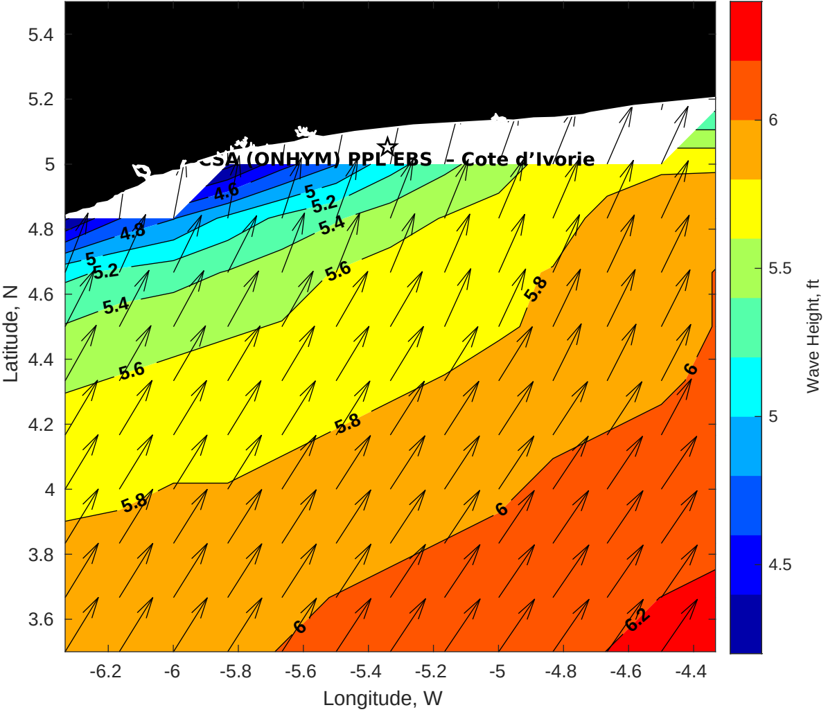
Wave Height (ft) for CSA (ONHYM) PPL EBS - Cote d'Ivoire at 04-Aug-2025 09:00:00
