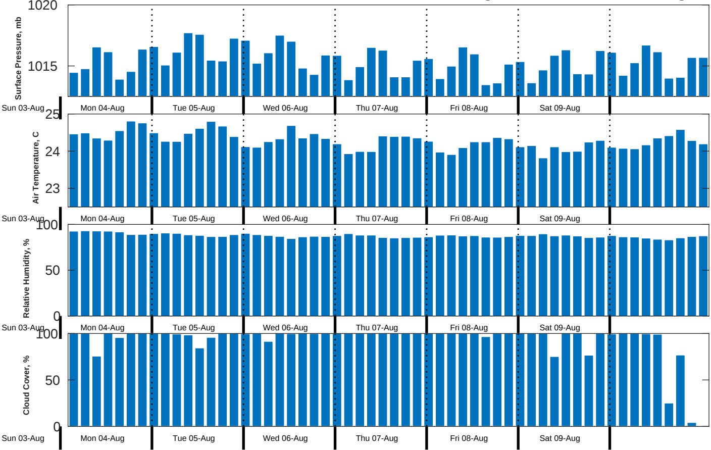
Met Forecast for CSA (ONHYM) PPL EBS - Cote d'Ivoire from 04-Aug-2025 00:00:00 to 11-Aug-2025 00:00:00
