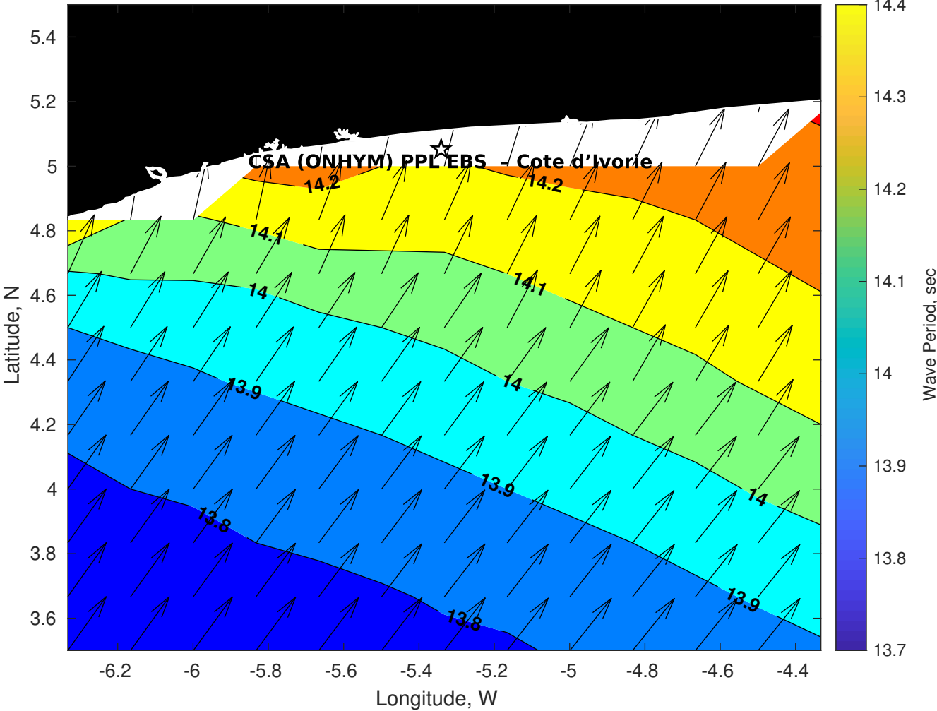
Wave Period (sec) for CSA (ONHYM) PPL EBS - Cote d'Ivoire at 04-Aug-2025 09:00:00
