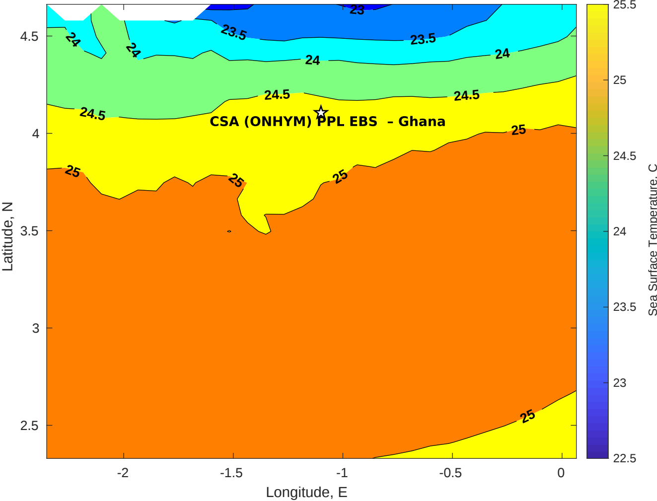
SST for CSA (ONHYM) PPL EBS - Ghana at 03-Aug-2025 00:00:00
