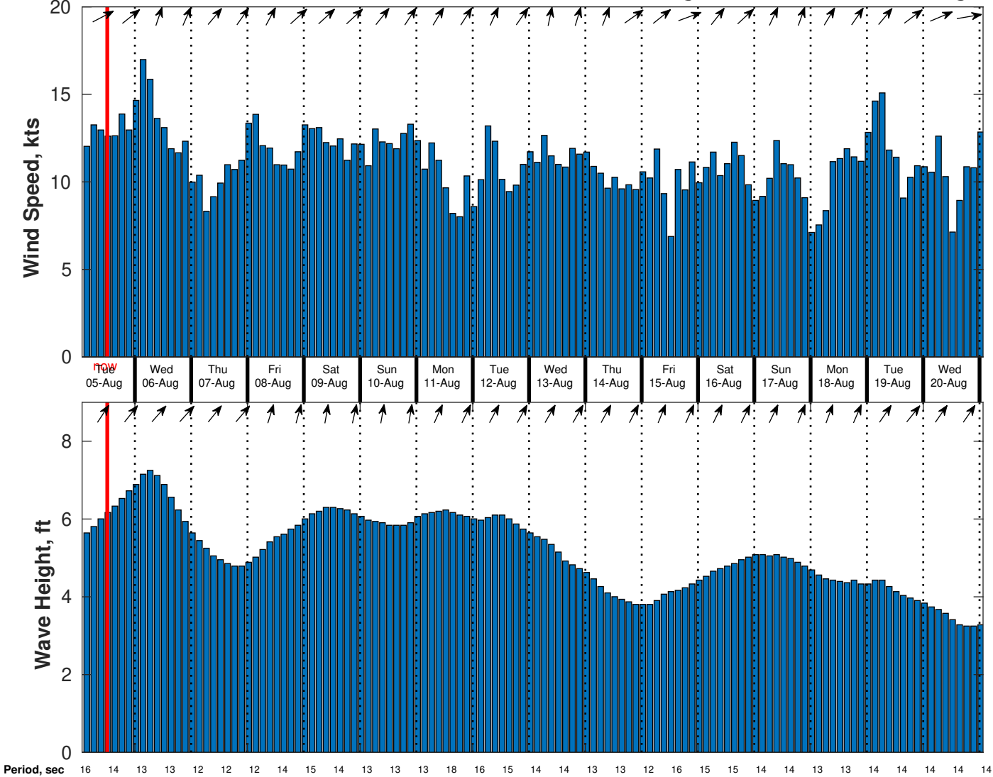
Wind & Wave Forecast for CSA (ONHYM) PPL EBS - Ghana from 04-Aug-2025 02:00:00 to 20-Aug-2025 02:00:00
