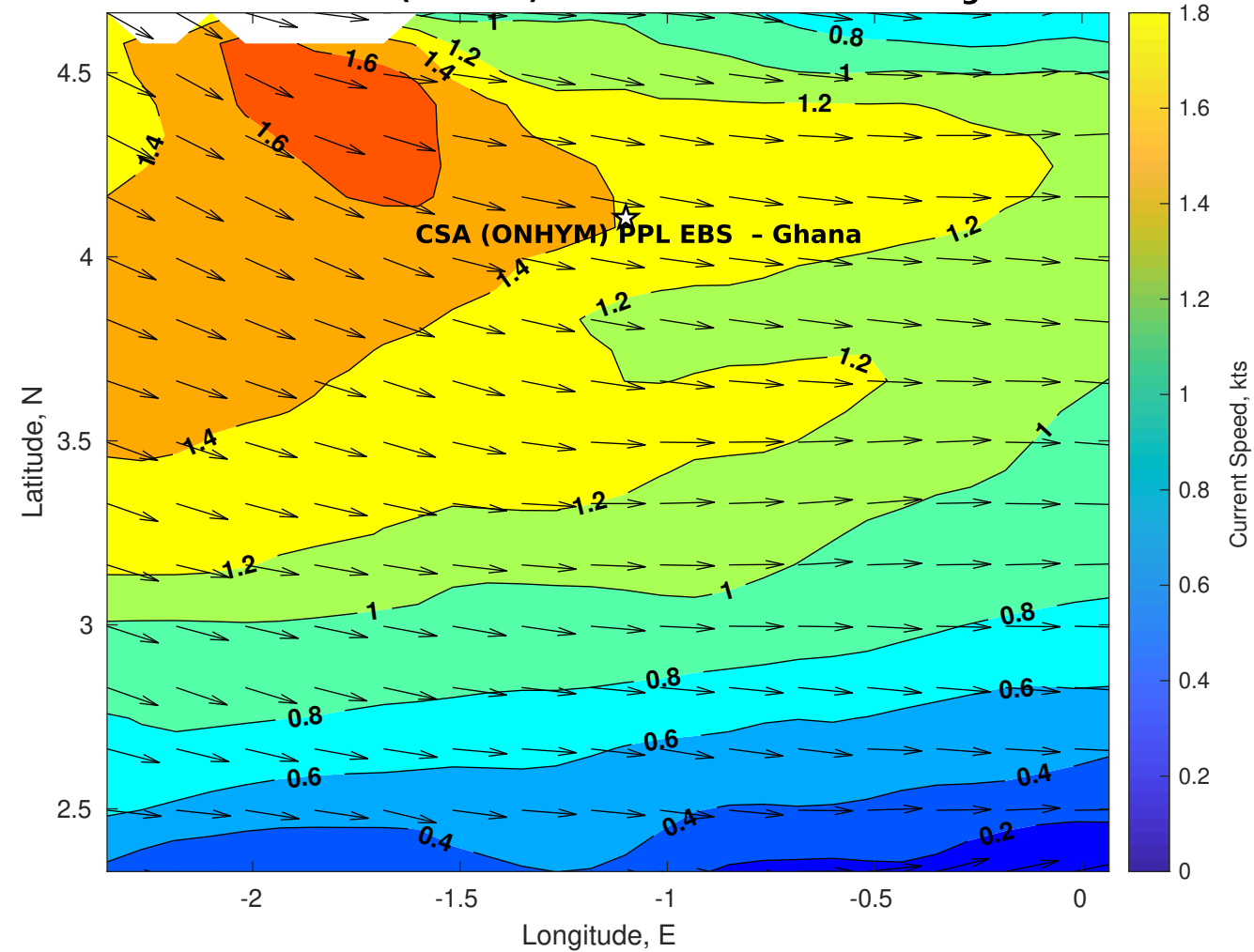
Surface Currents for CSA (ONHYM) PPL EBS - Ghana at 03-Aug-2025 00:00:00
