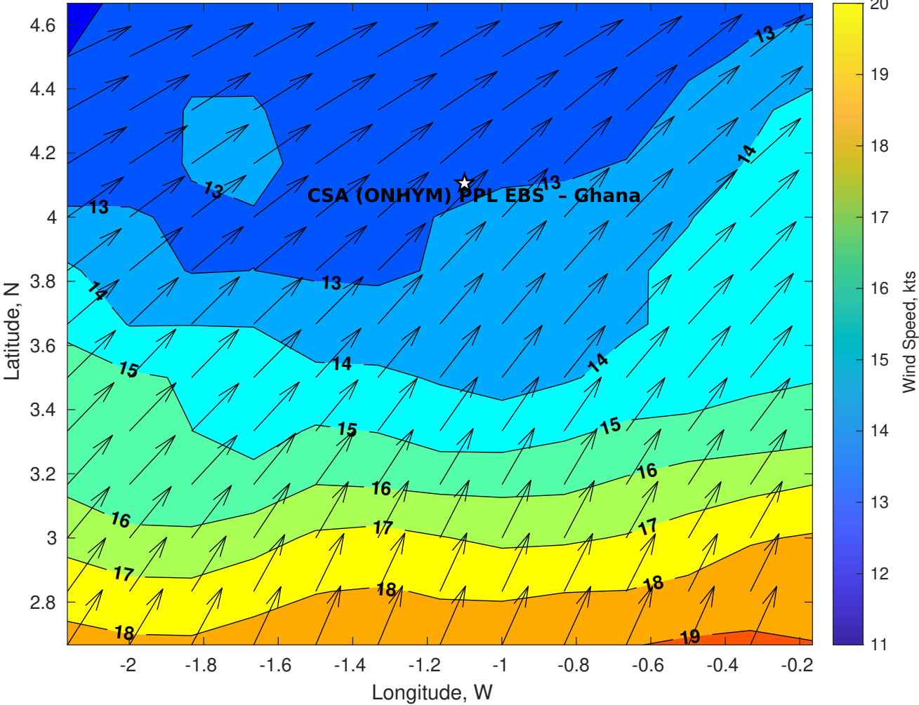
Winds (kts) for CSA (ONHYM) PPL EBS - Ghana at 04-Aug-2025 09:00:00
