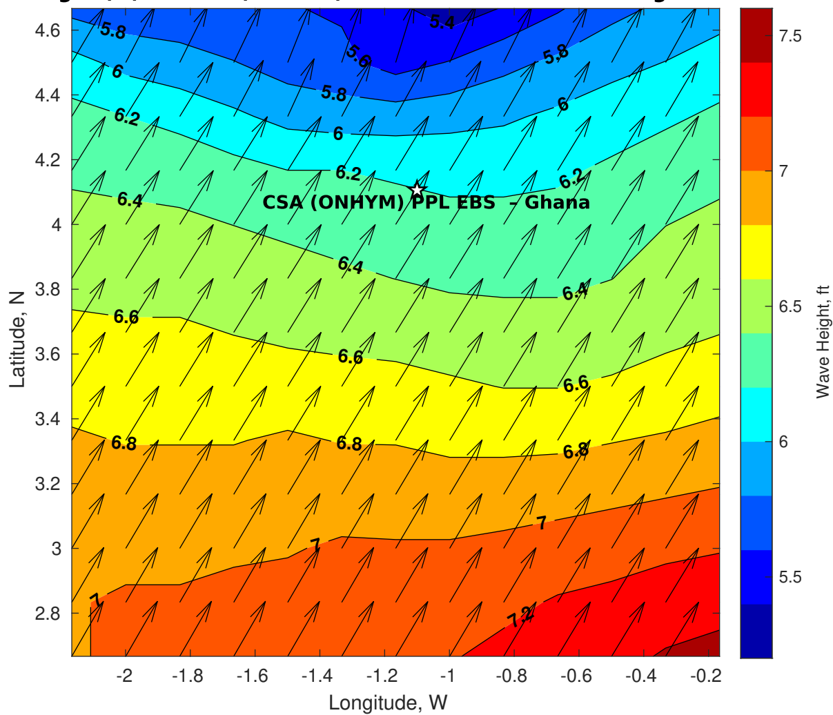
Wave Height (ft) for CSA (ONHYM) PPL EBS - Ghana at 04-Aug-2025 09:00:00
