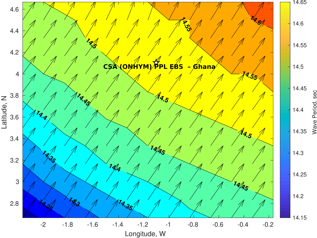
Wave Period (sec) for CSA (ONHYM) PPL EBS - Ghana at 04-Aug-2025 09:00:00
