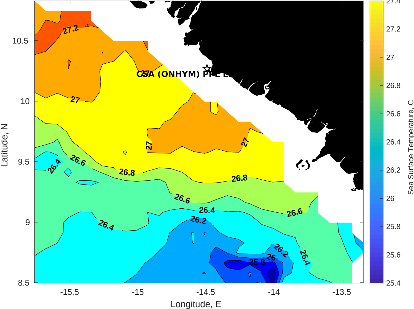
SST for CSA (ONHYM) PPL EBS - Guinea at 03-Aug-2025 00:00:00
