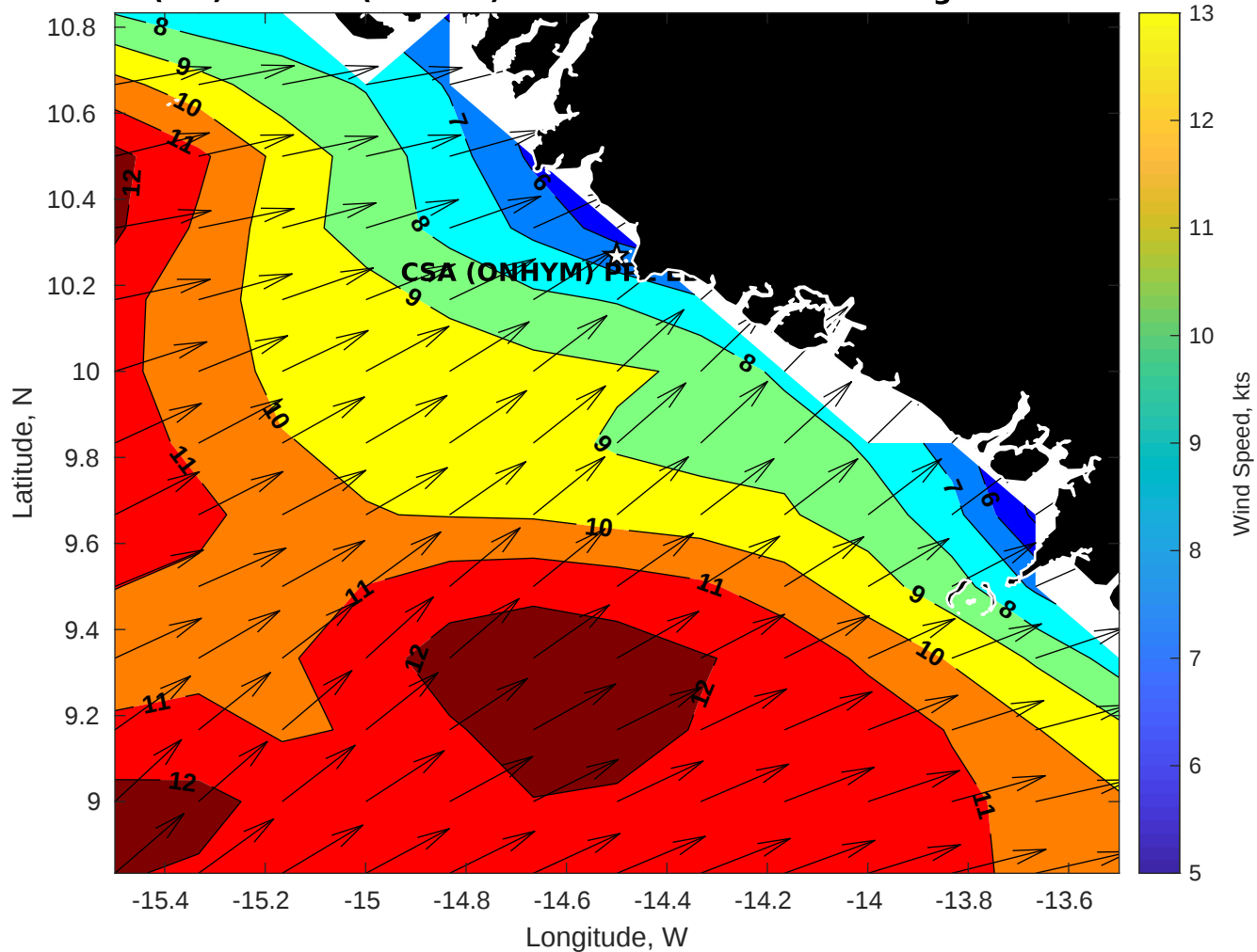
Winds (kts) for CSA (ONHYM) PPL EBS - Guinea at 04-Aug-2025 09:00:00
