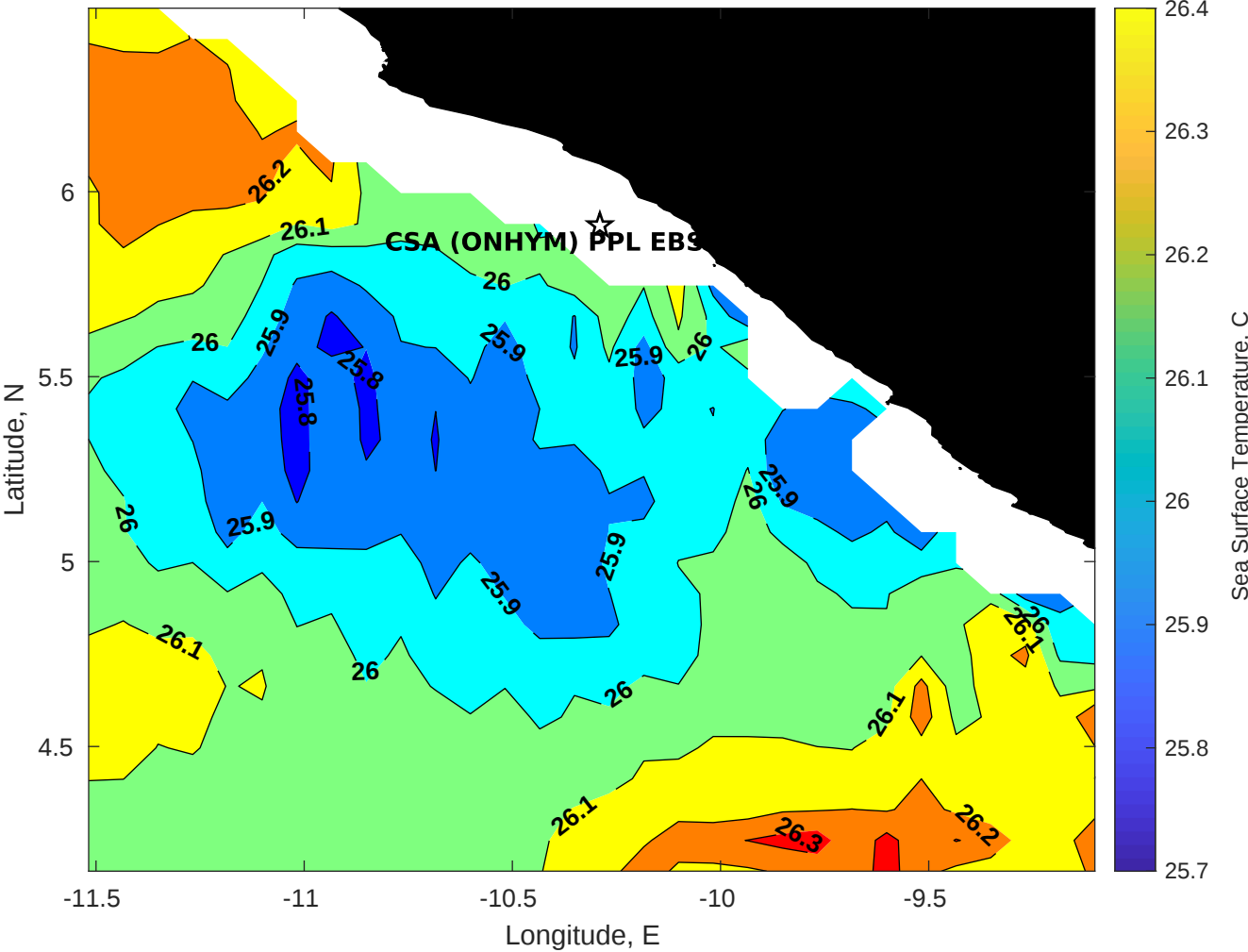
SST for CSA (ONHYM) PPL EBS - Liberia at 03-Aug-2025 00:00:00
