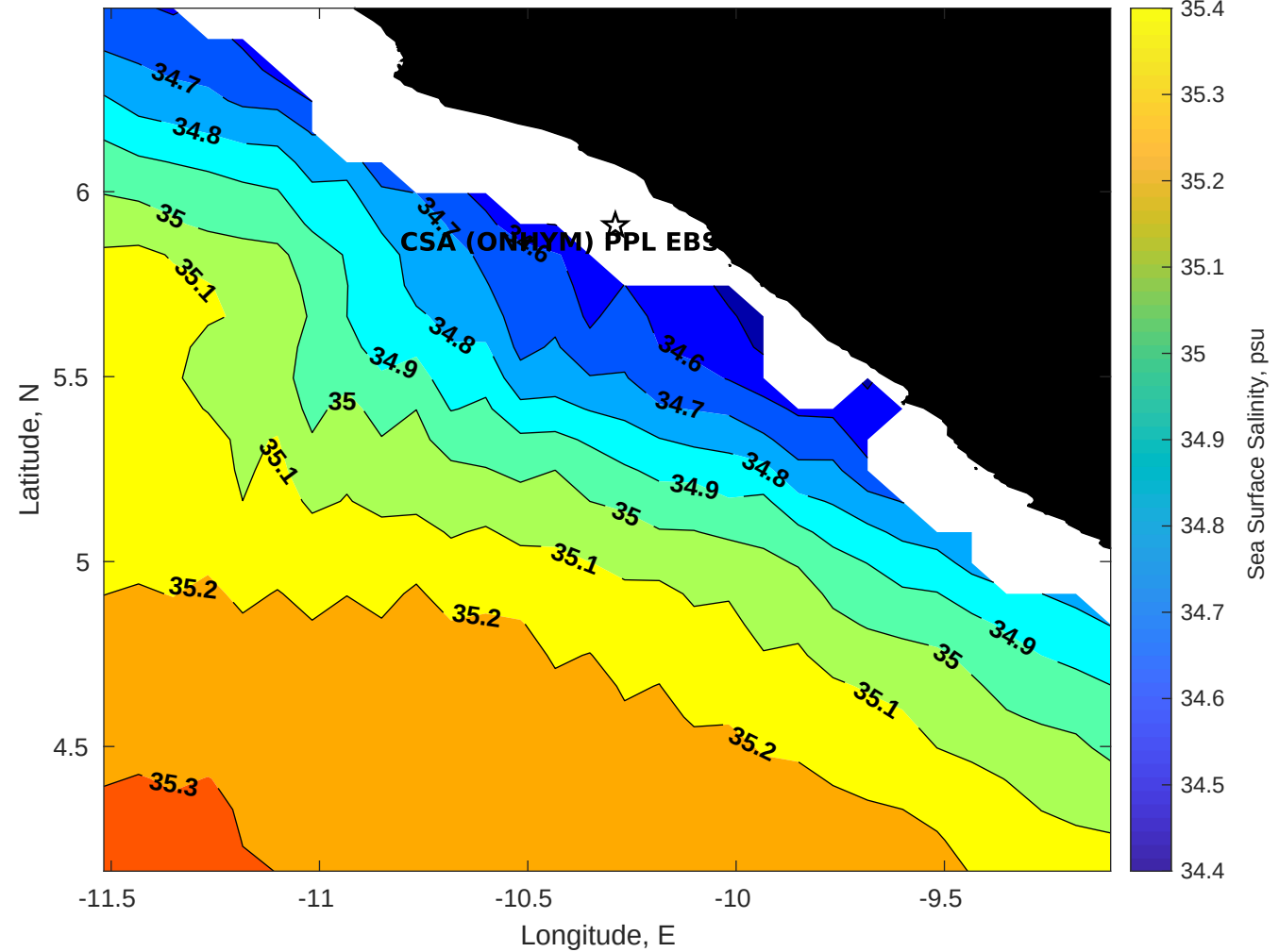
Surface Salinity for CSA (ONHYM) PPL EBS - Liberia at 03-Aug-2025 00:00:00
