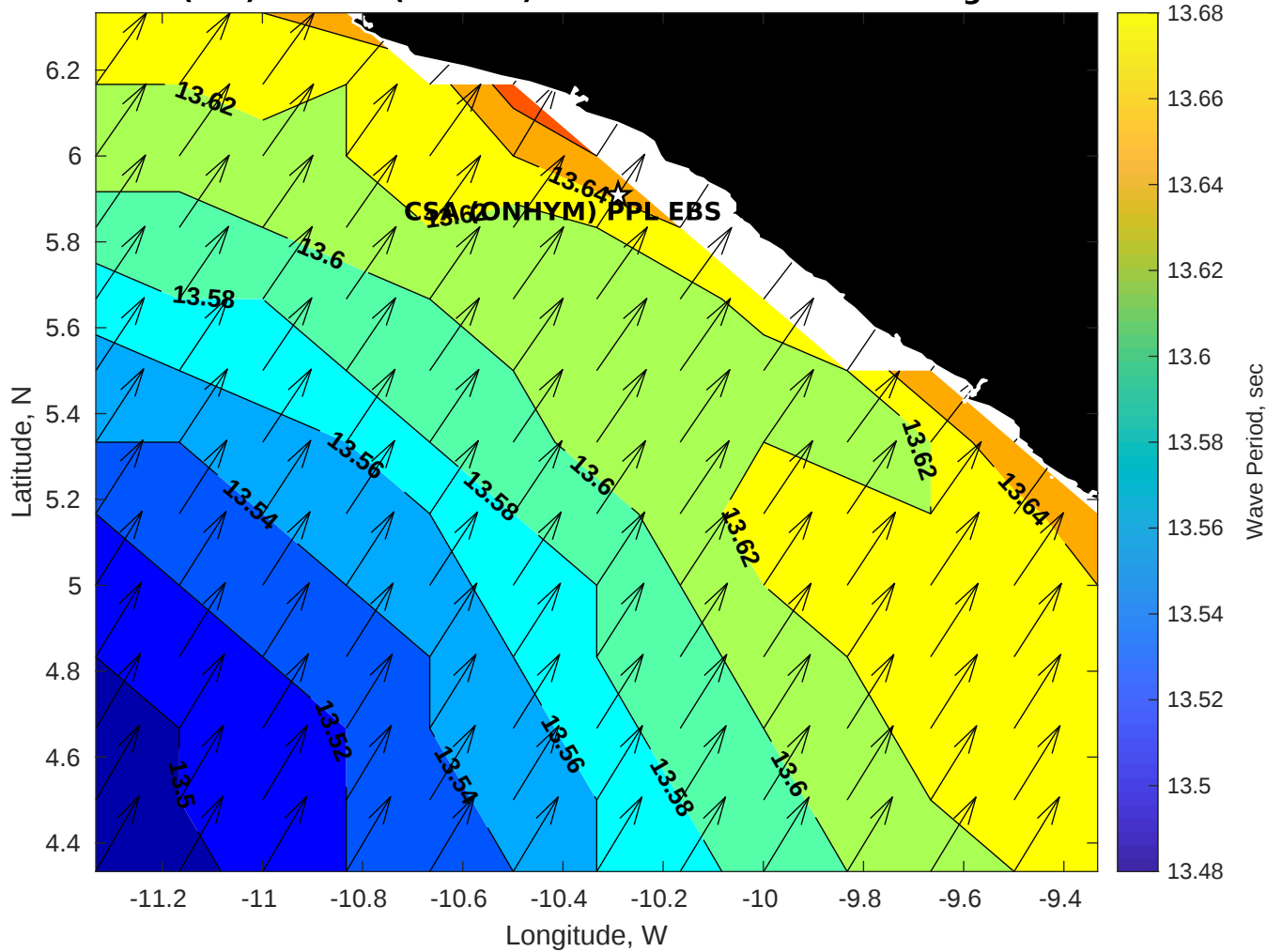
Wave Period (sec) for CSA (ONHYM) PPL EBS - Liberia at 04-Aug-2025 09:00:00
